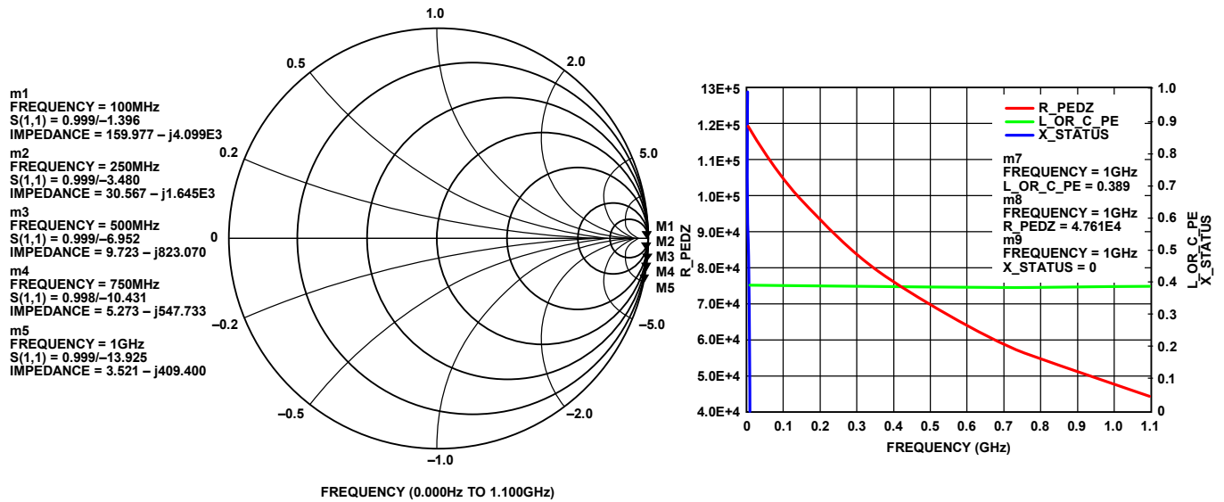
Figure 452. REF_CLK_IN± SEDZ and PEDZ Data, On Average, the Real Part of the Parallel Equivalent Differential Impedance ( R_P ) = Approximately 70 k \Omega
