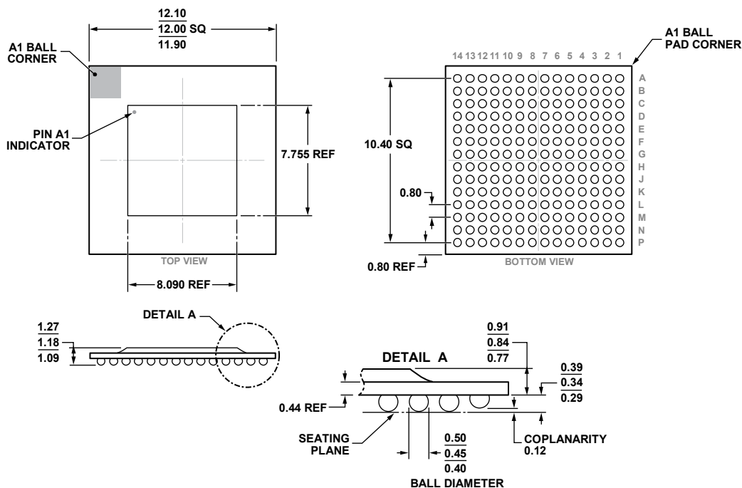
COMPLIANT TO JEDEC STANDARDS MO-275-GGAB-1. Figure 466. 196-Ball Chip Scale Package Ball Grid Array [CSP_BGA] (BC-196-13) Dimensions shown in millimeters
