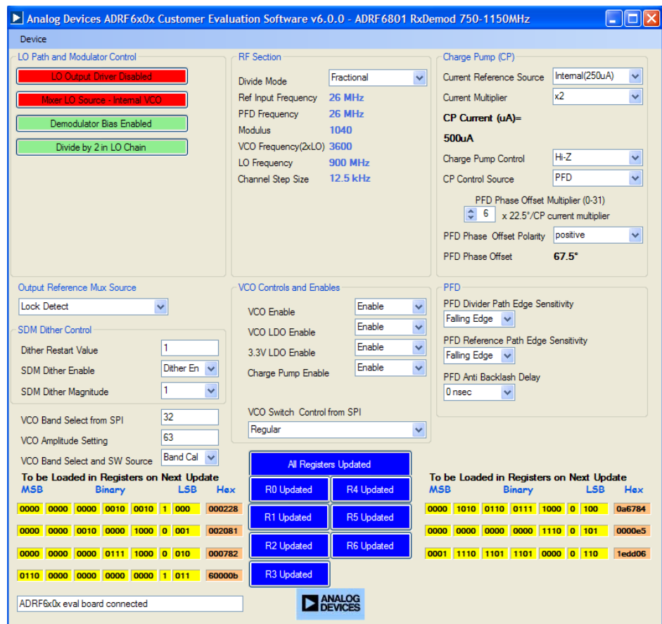
Figure 46. Evaluation Board Software Main Window
