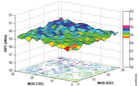
Figure 53. OIP2 vs. MOD_CSEL and MOD_RSEL at f_{RF} = 2140 MHz, I/Q Amplitude per Tone = 0.3 V p-p Differential
