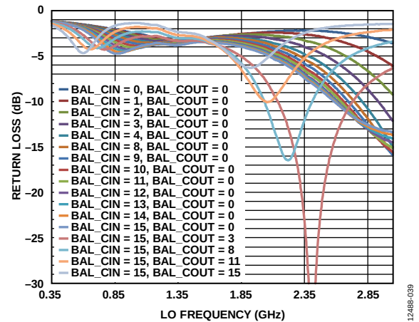
Figure 39. RF Output Return Loss vs. LO Frequency ( f_{o} ) for Multiple BAL_CIN and BAL_COUT Combinations
