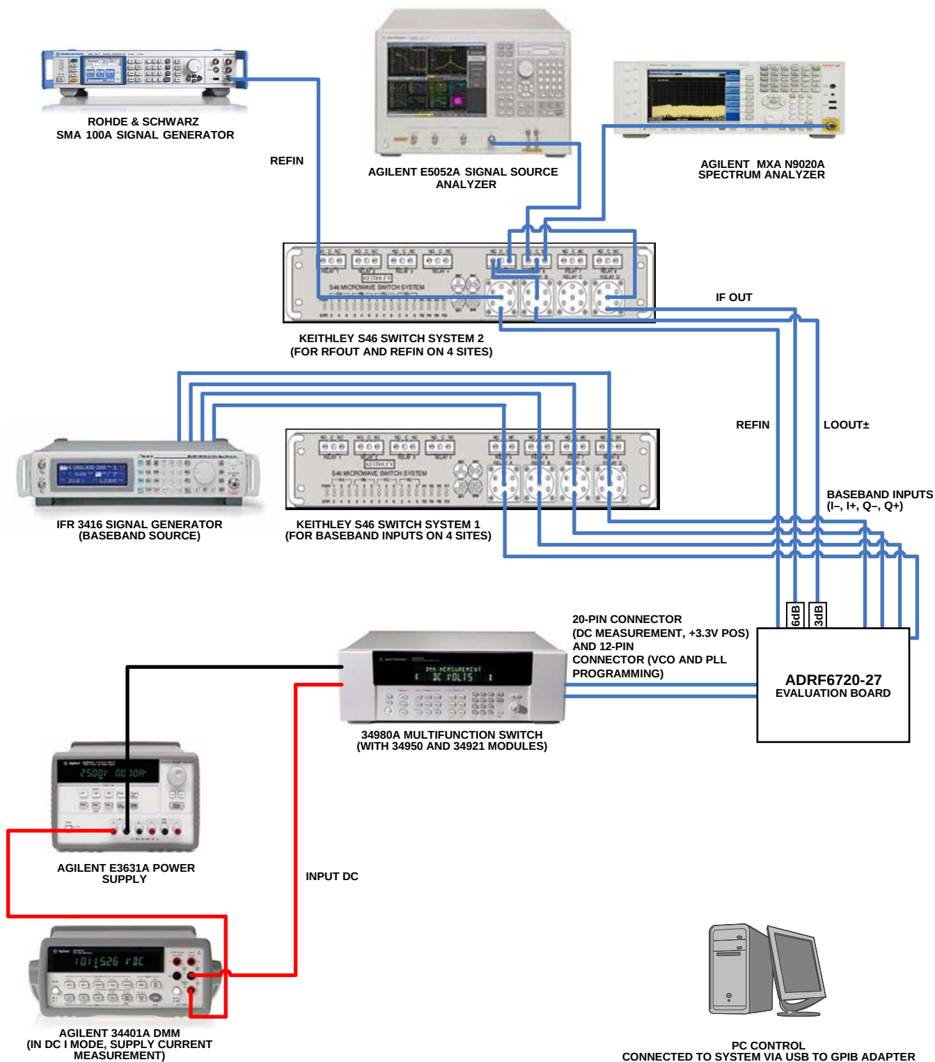
Figure 63. Characterization Setup for Phase Noise and Reference Spur Measurements
