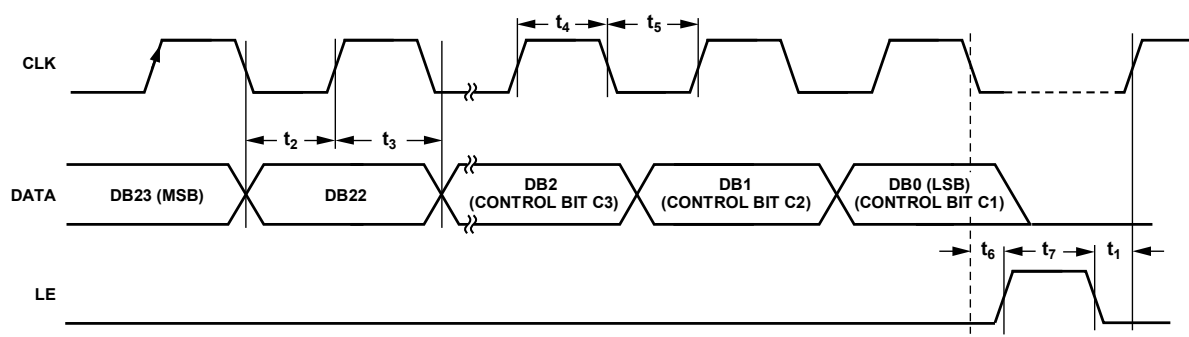
Figure 2. Timing Diagram
