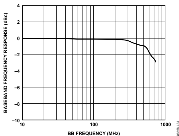
Figure 39. Baseband Bandwidth
