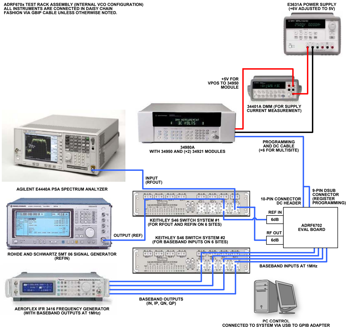
Figure 49. General Characterization Setup
