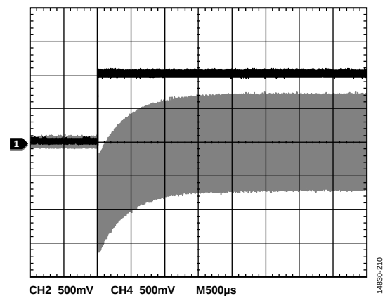
Figure 72. VGA2 Gain Step Response; C9 or C16 = 1 \mu\text{F}
