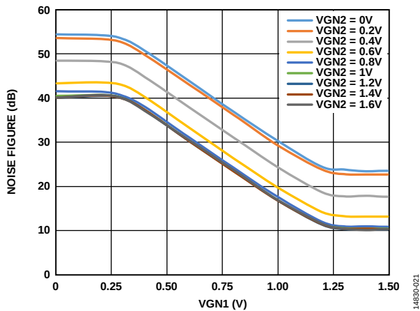
Figure 27. Noise Figure vs. VGN1 over VGN2, Bypass Mode
