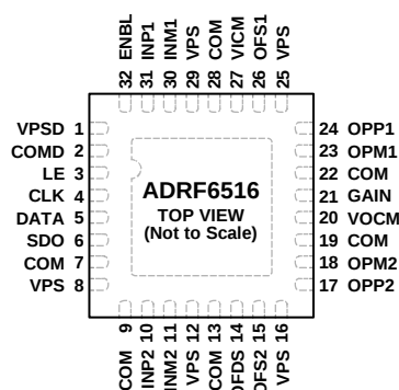
Figure 4. Pin Configuration
