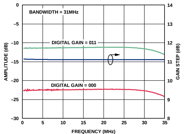
Figure 10. Gain Step and Gain Error vs. Frequency (Bandwidth Setting = 31 MHz, V_{\text{GAIN}} = 0\text{ V} )
