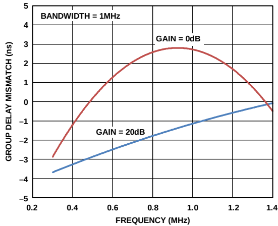
Figure 17. IQ Group Delay Matching vs. Frequency (Bandwidth Setting = 1 MHz)
