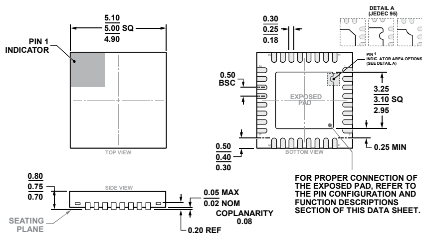
Figure 62. 32-Lead Lead Frame Chip Scale Package [LFCSP] 5 mm x 5 mm Body and 0.75 mm Package Height (CP-32-7)
