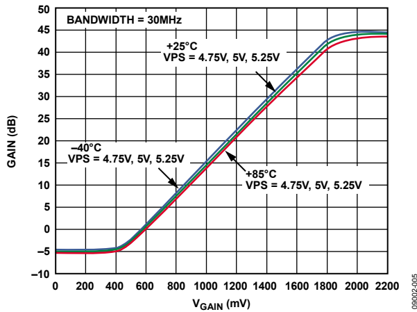
Figure 5. In-Band Gain vs. V GAIN over Supply and Temperature (Bandwidth Setting = 30 MHz)
