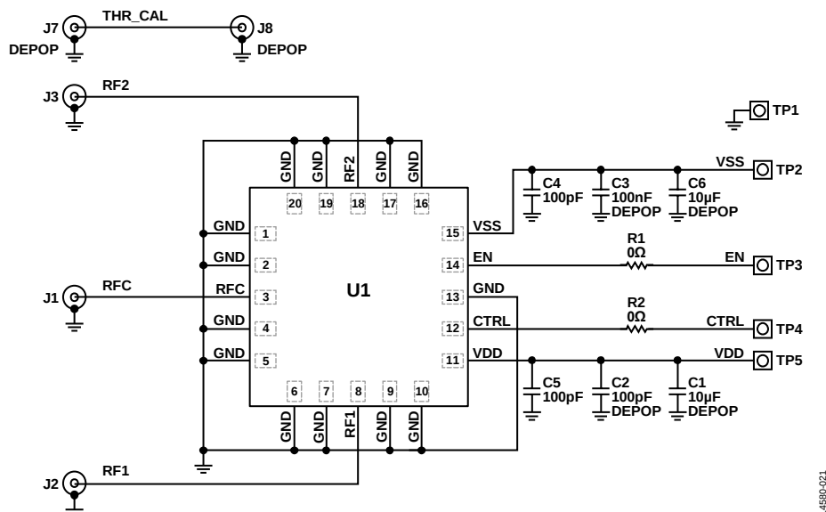
Figure 21. Evaluation Board Schematic
