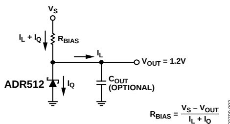
Figure 2. Typical Operating Circuit
