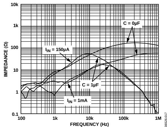
Figure 17. ADR5045 Output Impedance vs. Frequency
