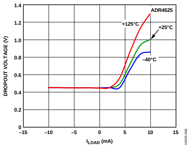
Figure 22. ADR4525 Dropout Voltage vs. Load Current
