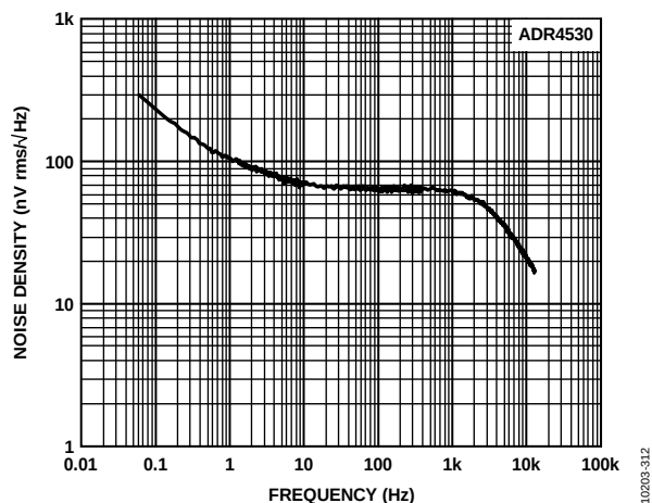
Figure 47. ADR4530 Output Noise Spectral Density
