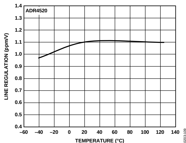
Figure 10. ADR4520 Line Regulation vs. Temperature
