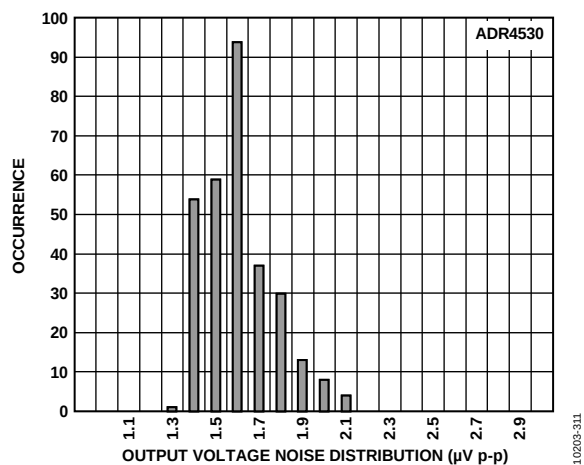
Figure 46. ADR4530 Output Voltage Noise (Maximum Amplitude from 0.1 Hz to 10 Hz)
