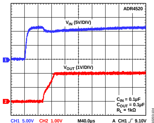
Figure 6. ADR4520 Output Voltage Start-Up Response
