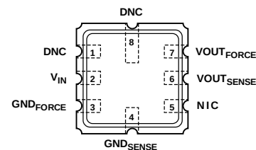
Figure 2. 8-Lead LCC Pin Configuration
