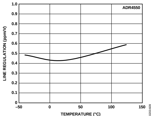
Figure 93. ADR4550 Line Regulation vs. Temperature
