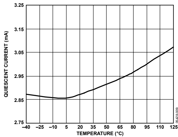
Figure 11. ADR445 Quiescent Current vs. Temperature
