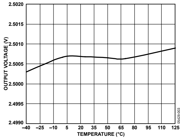
Figure 3. ADR441 Output Voltage vs. Temperature
