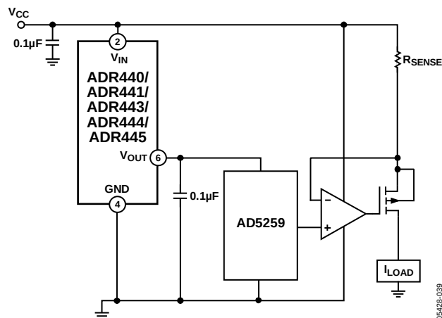
Figure 38. Programmable Current Source
