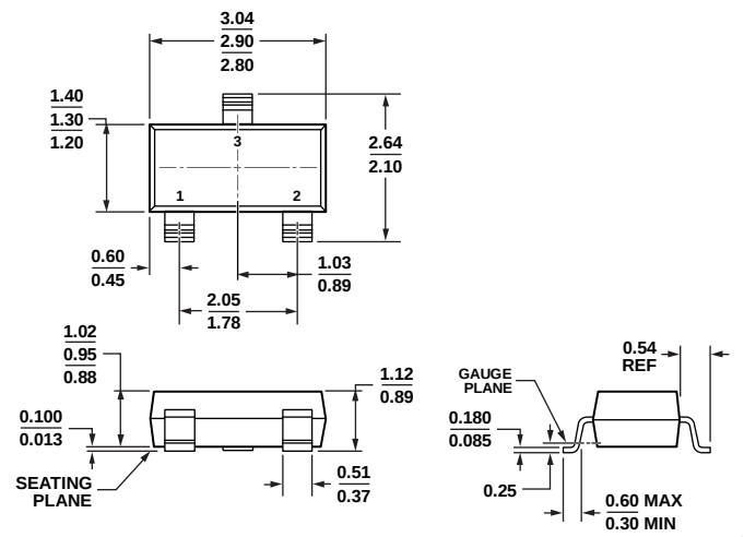
COMPLIANT TO JEDEC STANDARDS TO-236-AB Figure 31. 3-Lead Small Outline Transistor Package [SOT-23-3] (RT-3) Dimensions shown in millimeters
