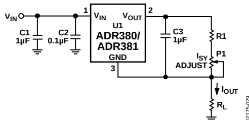
Figure 29. Precision Current Source
