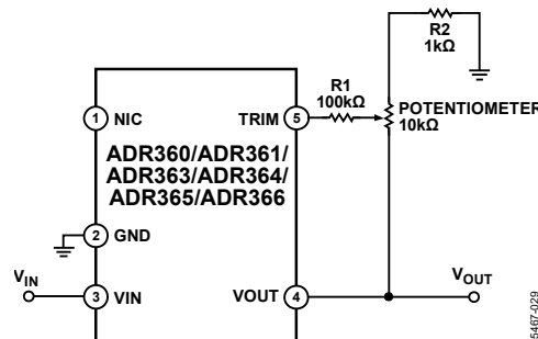
Figure 40. ADR360/ADR361/ADR363/ADR364/ADR365/ADR366 Trim Configuration
