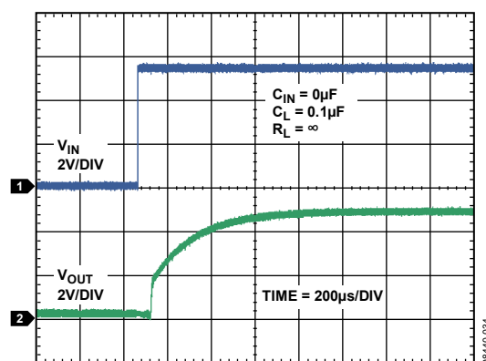
Figure 25. ADR3450 Start-Up Response
