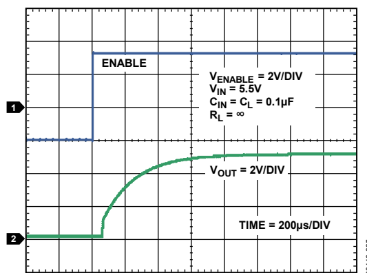
Figure 26. ADR3450 Restart Response from Shutdown
