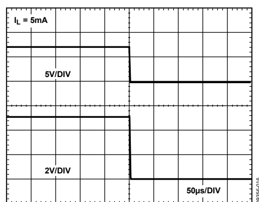
Figure 12. Turn-Off Time
