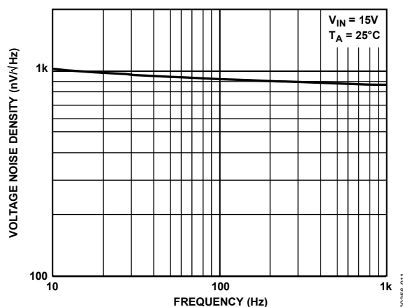
Figure 7. Voltage Noise Density vs. Frequency
