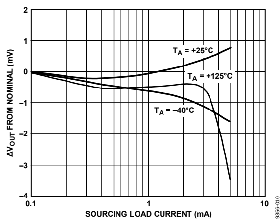
Figure 6. \Delta V_{OUT} from Nominal vs. Load Current
