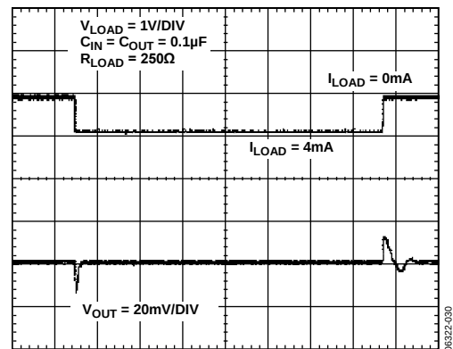
Figure 30. Load Transient Response (Source), V_{OUT} = 1\text{ V}
