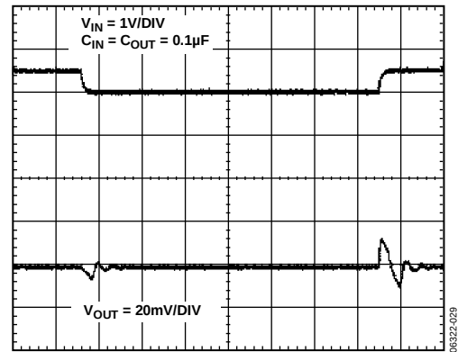
Figure 29. Line Transient Response, V_{OUT} = 1\text{ V}
