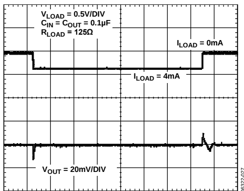
Figure 27. Load Transient Response (Source), V_{OUT} = 0.5\text{ V}
