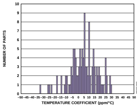
Figure 3. Temperature Coefficient, V_{OUT} = 0.5\text{ V}
