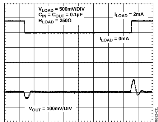
Figure 31. Load Transient Response (Sink), V_{OUT} = 1\text{ V}
