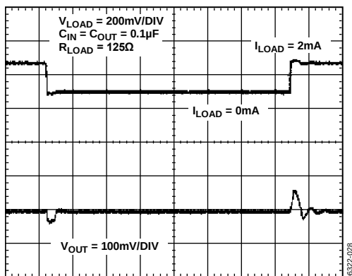
Figure 28. Load Transient Response (Sink), V_{OUT} = 0.5\text{ V}
