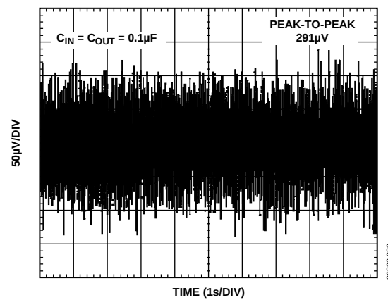
Figure 23. 10 Hz to 10 kHz Noise, V_{OUT} = 1\text{ V}
