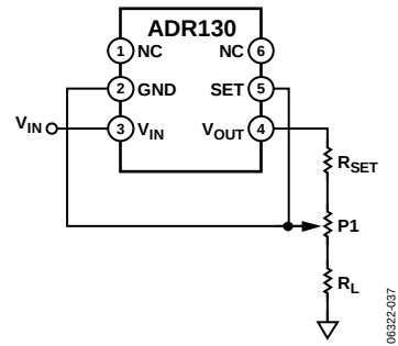
Figure 36. ADR130 as a Precision Current Source
