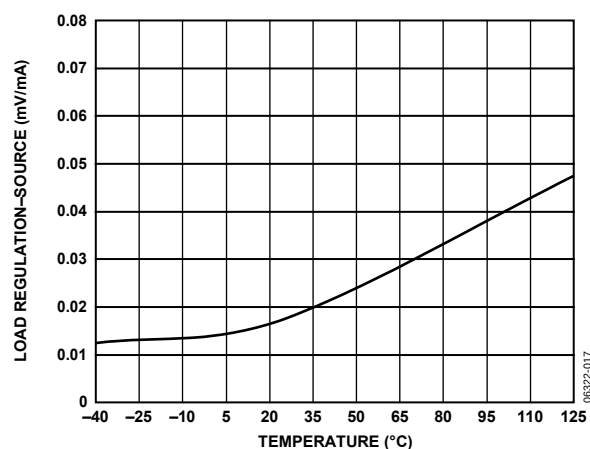
Figure 17. Load Regulation (Source) vs. Temperature, V_{OUT} = 1\text{ V}
