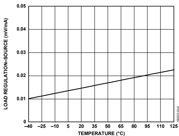
Figure 14. Load Regulation (Source) vs. Temperature, V_{OUT} = 0.5\text{ V}
