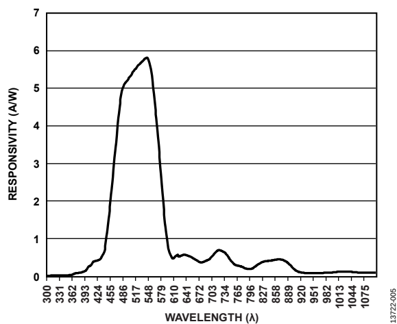
Figure 5. Responsivity vs. Wavelength
