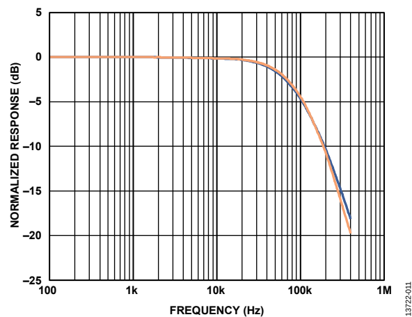
Figure 9. Bandwidth/Peaking
