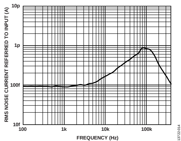
Figure 10. Noise Bandwidth/Peaking
