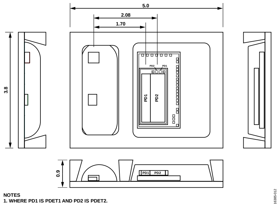
Figure 21. Optical Component Locations
