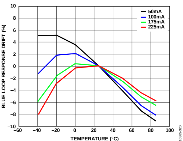
Figure 20. Blue Loop Response Drift vs. Temperature
