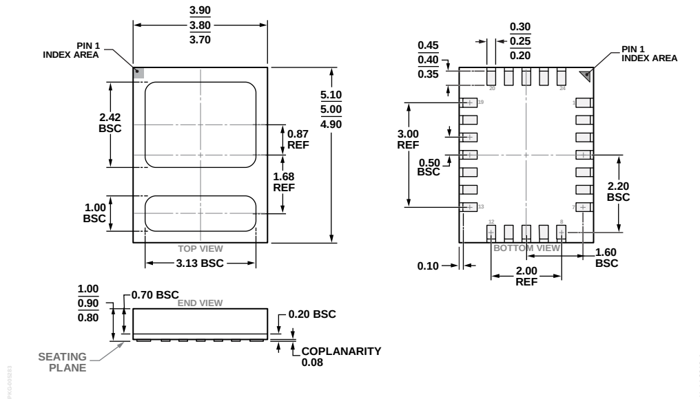
Figure 47. 24-Terminal Chip Array Small Outline No Lead Cavity [LGA_CAV] 3.80 mm x 5.00 mm Body and 0.9 mm Package Height (CE-24-1) Dimensions shown in millimeters
