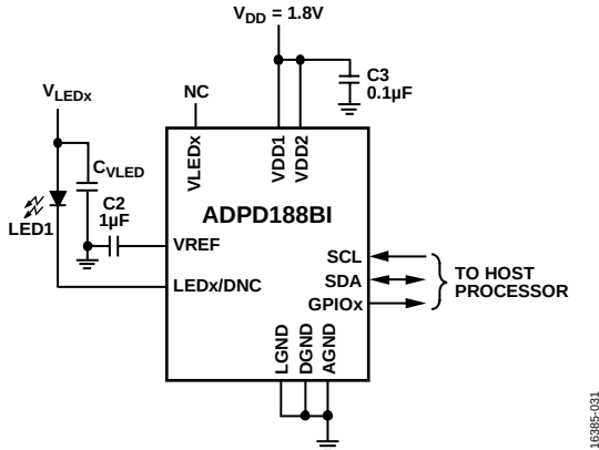
Figure 38. Using the ADPD188BI LED Drivers to Drive External LEDs
