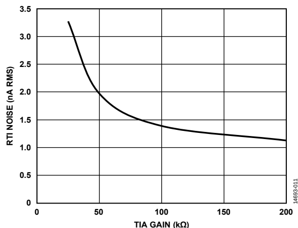
Figure 14. Referred to Input (RTI) Noise vs. TIA Gain
