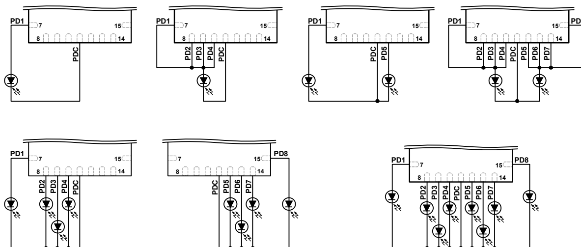
Figure 37. Photodiode Configuration Options for the ADPD105 LFCSP
