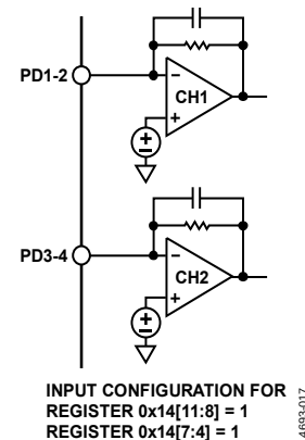
Figure 23. Current Summation—Two Photodiodes Summed into One Current
