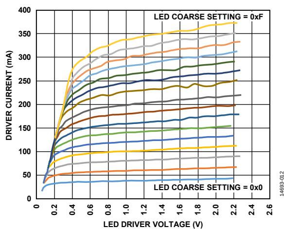
Figure 15. LED Driver Current vs. LED Driver Voltage at Various Coarse Settings
