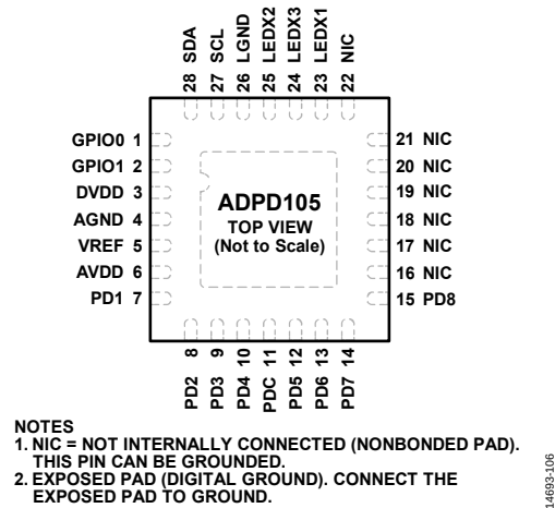
Figure 6. 28-Lead LFCSP Pin Configuration (ADPD105)
