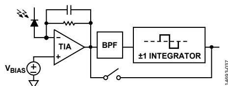
Figure 44. Signal Path Block Diagram
