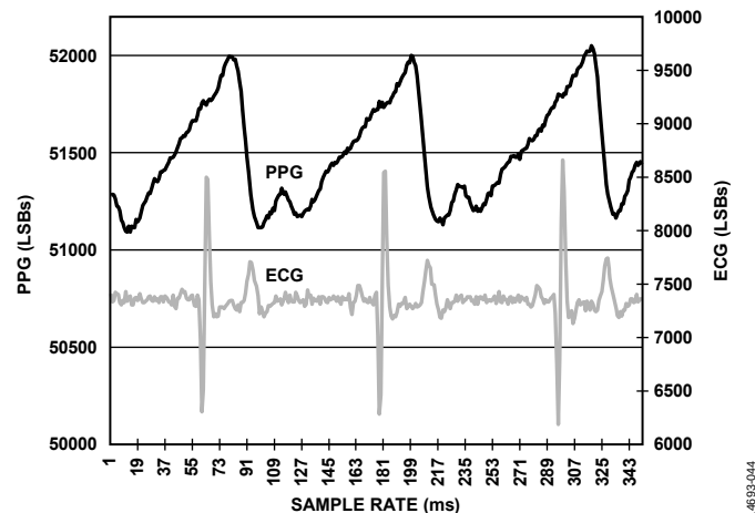
Figure 51. Plot of Synchronized ECG and PPG Waveforms
