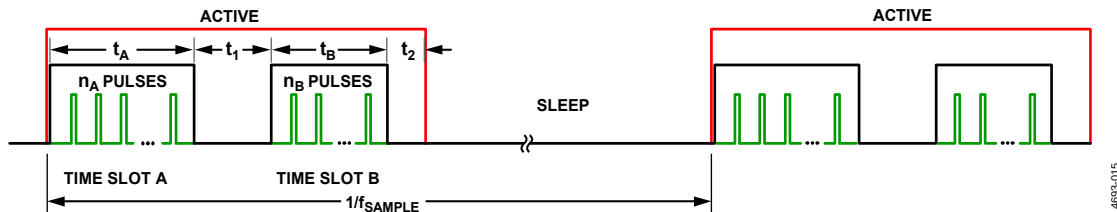
Figure 18. Time Slot Timing Diagram
