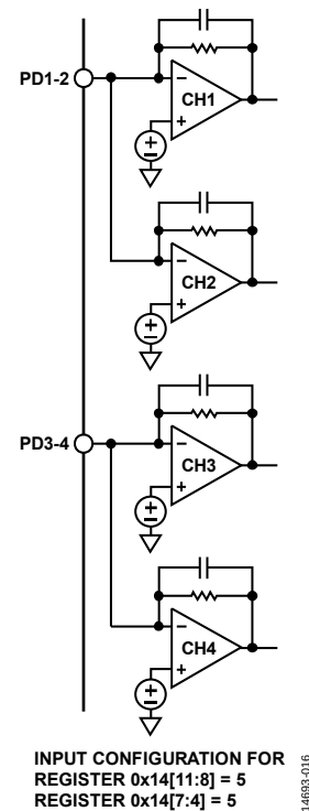
Figure 22. PD1 to PD4 Connection
