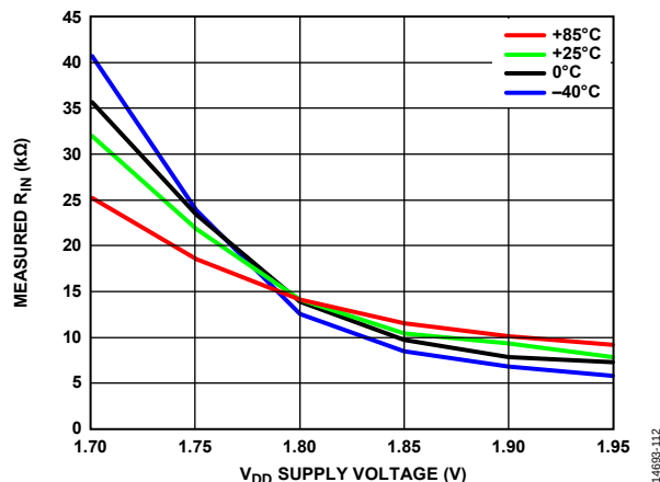
Figure 53. Variability of Switch Input Resistance as a Function of V_{DD} Supply Voltage
