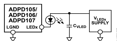
Figure 38. V_{LEDx} Supply Schematic
