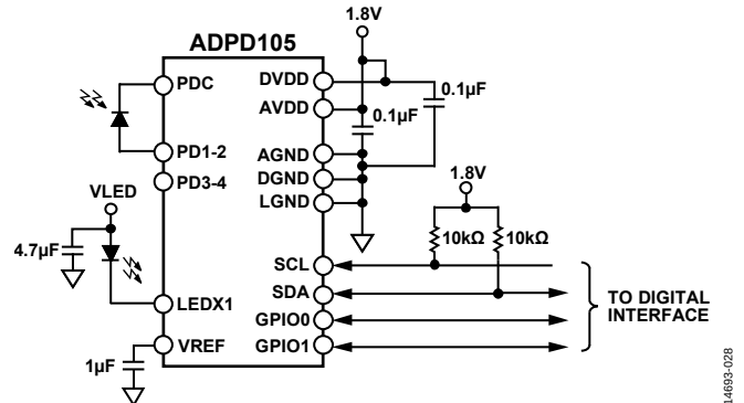
Figure 34. Typical Wrist-Based HRM Measurement
