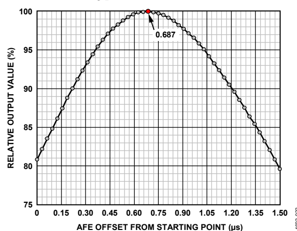
Figure 28. AFE Sweep Example
