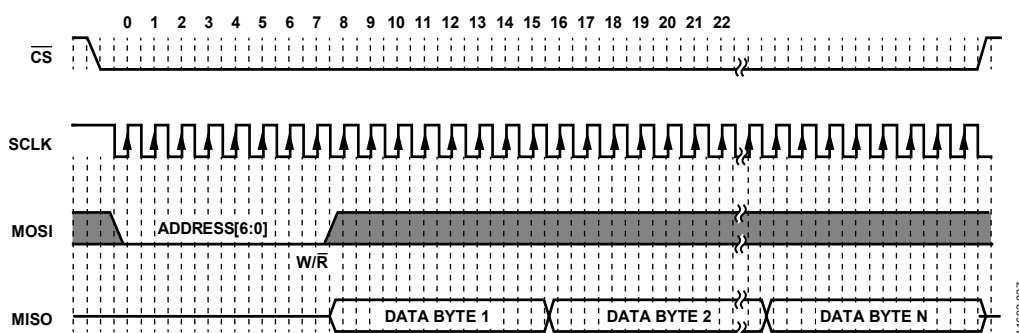
Figure 33. SPI Slave Read Clocking (Burst Read Mode, N Bytes)
