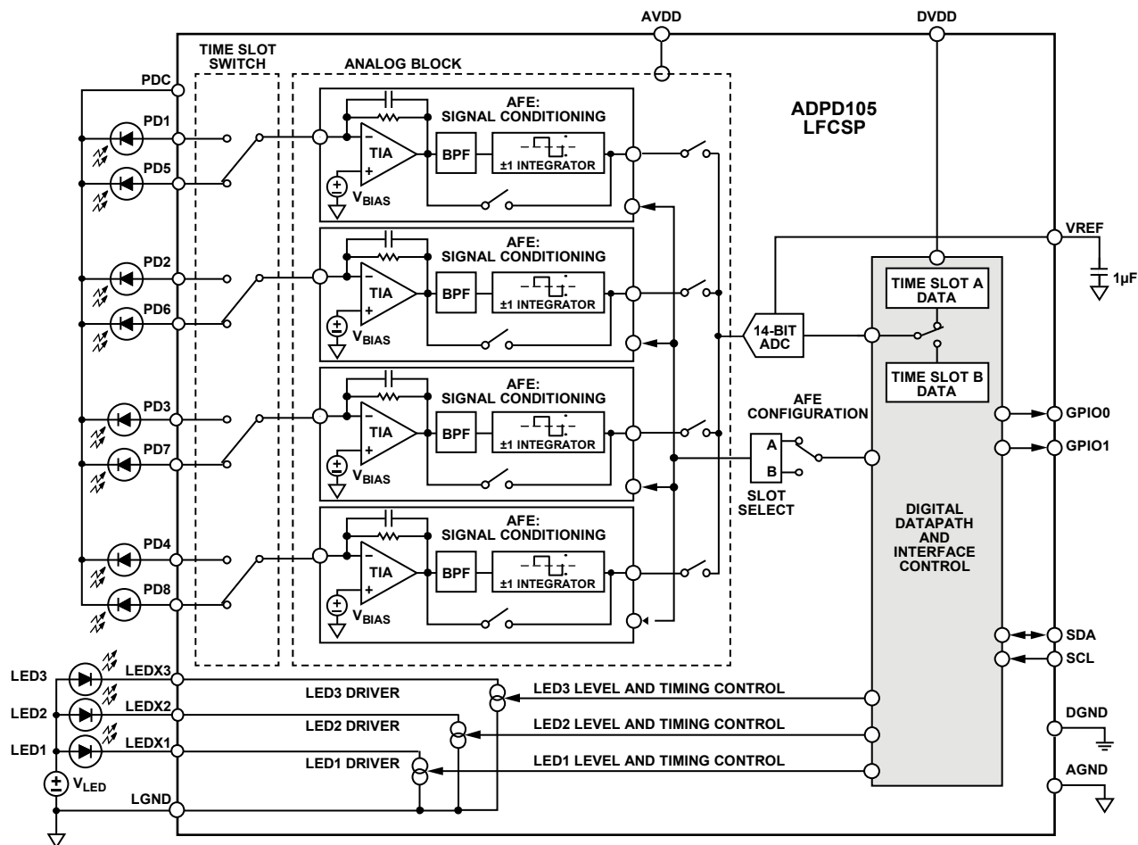
Figure 2. Block Diagram for ADPD105 LFCSP Version
