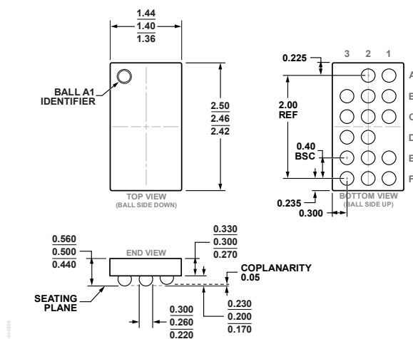
Figure 55. 16-Ball Wafer Level Chip Scale Package [WLCSP] (CB-16-18)
