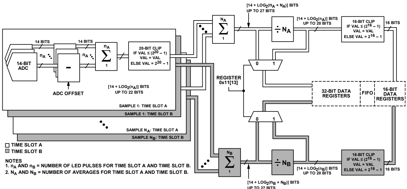
Figure 25. ADPD105/ADPD106/ADPD107 Datapath
