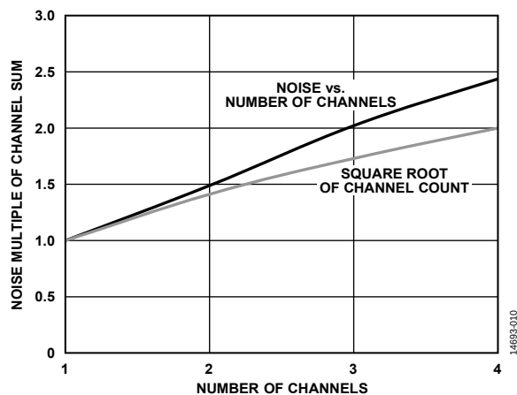
Figure 13. Noise Multiple of Channel Sum vs. Number of Channels
