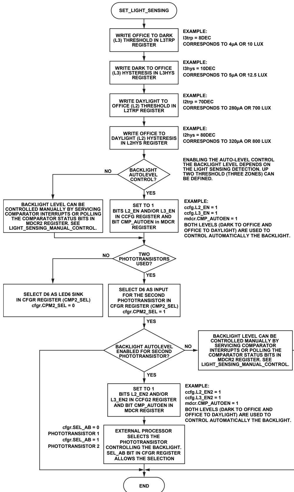
Figure 20. Set Light Sensing Flowchart
