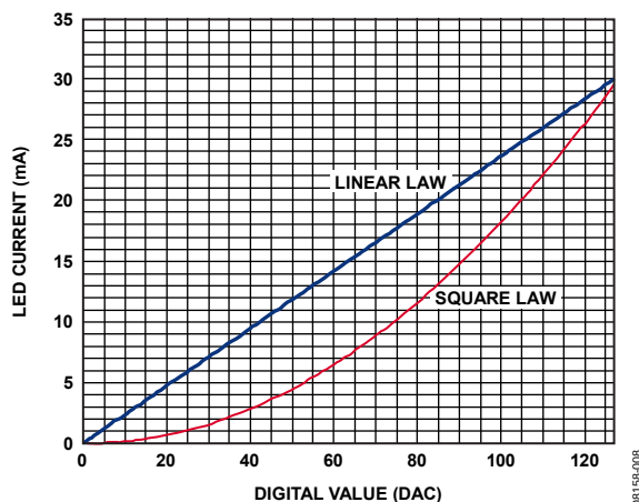
Figure 8. LED Current Transfer Law Curves
