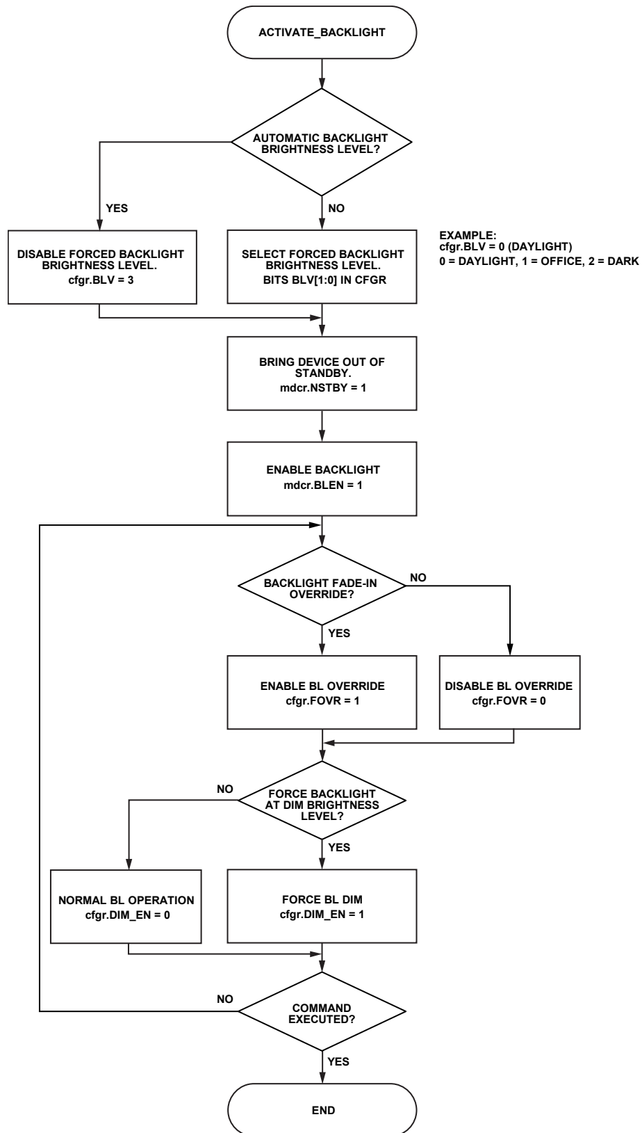
Figure 14. Activate Backlight Flowchart
