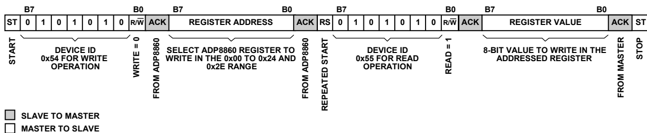
Figure 4. I 2 C Read Operation
