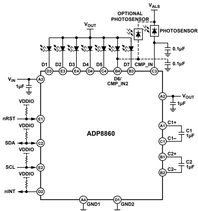
Figure 1. Typical Application Schematic with Optional Second Photo Diode
