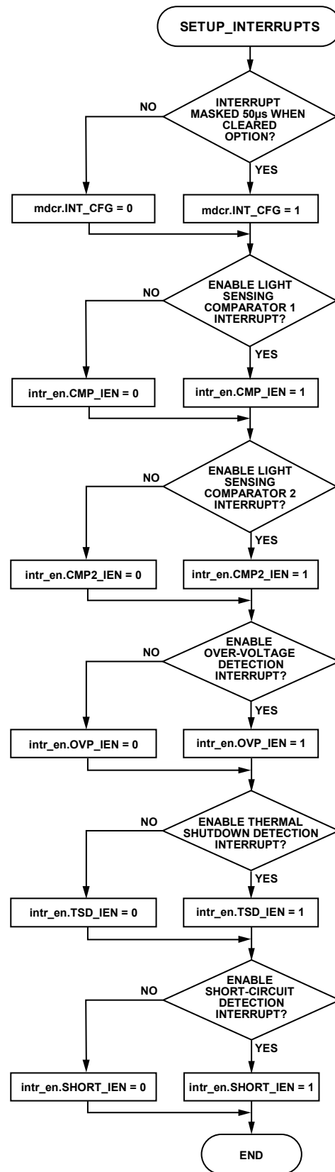
Figure 18. Setup Interrupts Flowchart
