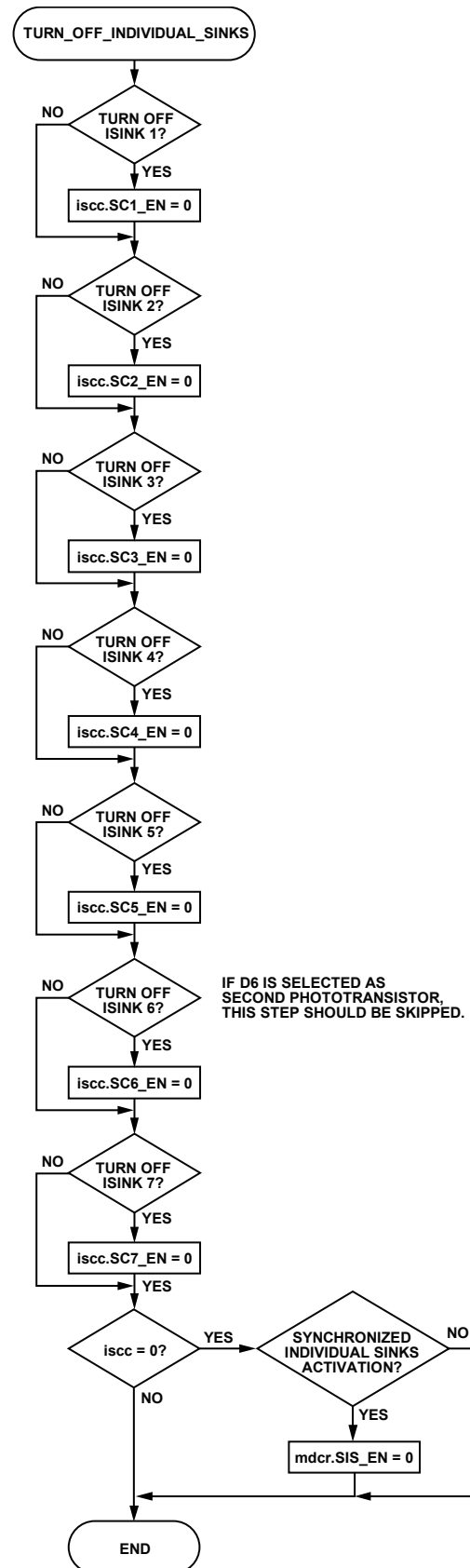
Figure 17. Turn Off Individual Sinks Flowchart
