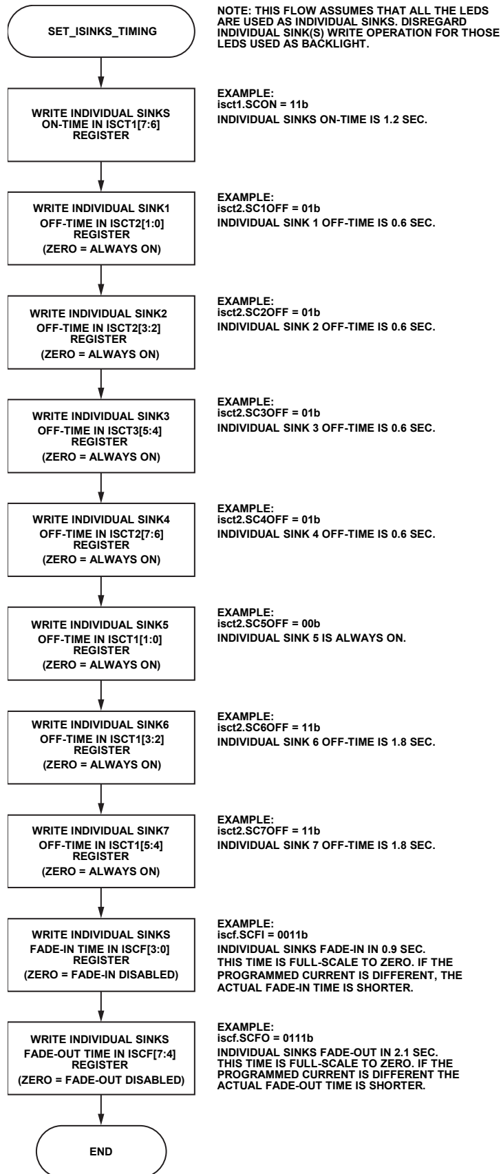
Figure 13. Set ISINKS Timing Flowchart
