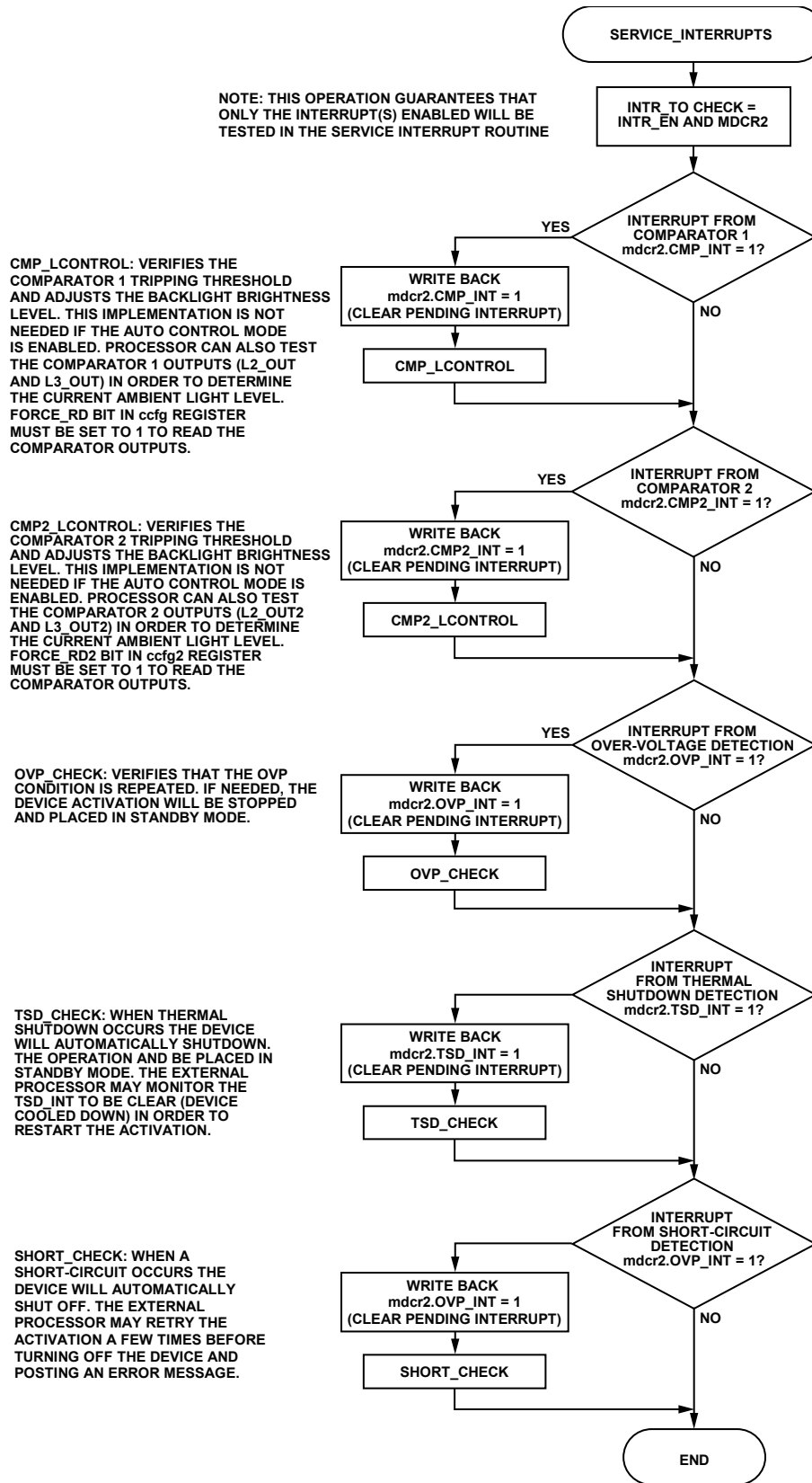
Figure 19. Service Interrupts Flowchart
