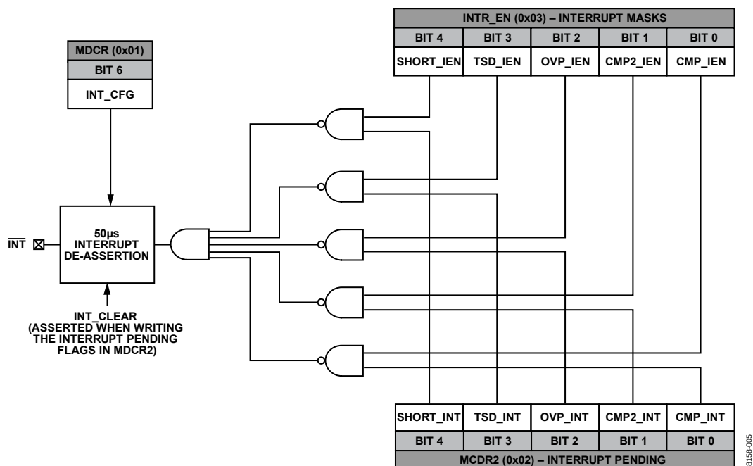
Figure 5. Interrupt Logic
