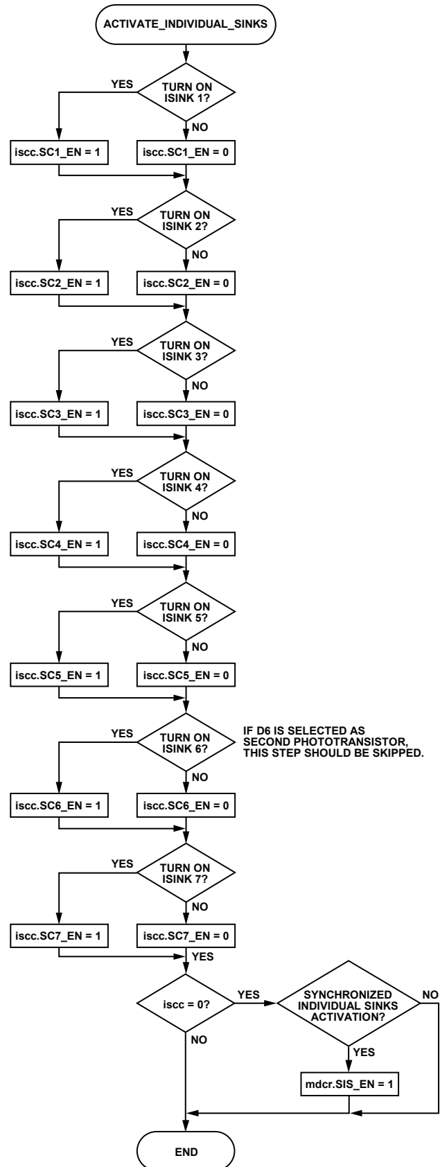
Figure 16. Activate Individual Sinks Flowchart
