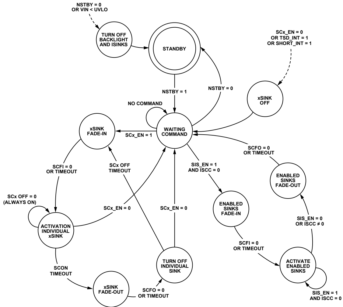
Figure 7. Individual Sinks Data Flow
