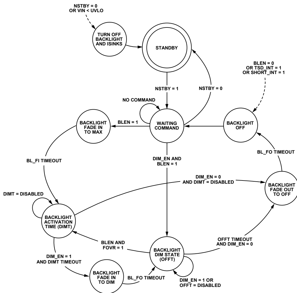
Figure 6. Backlight Data Flow
