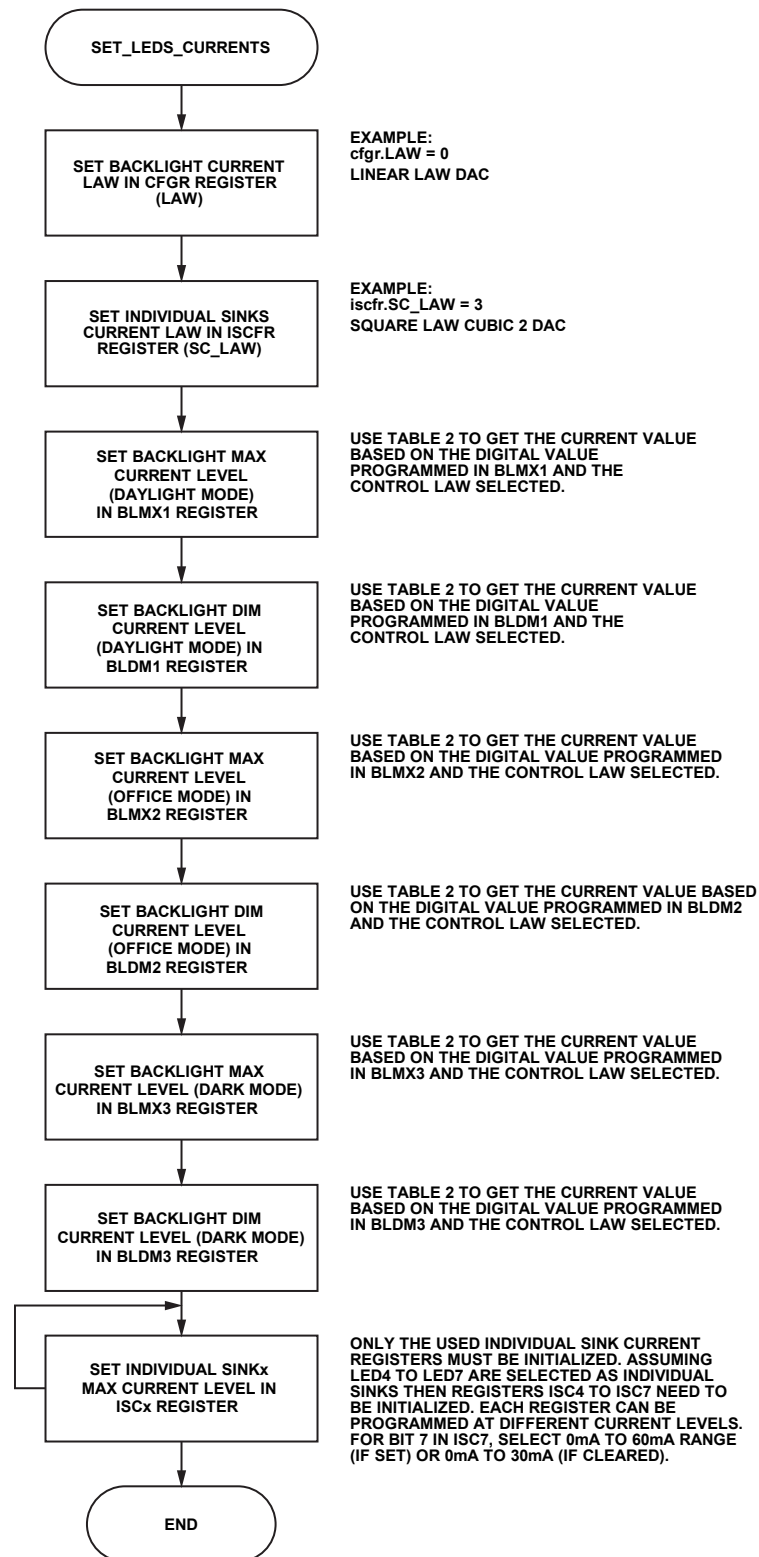
Figure 12. Set LEDs Currents Flowchart
