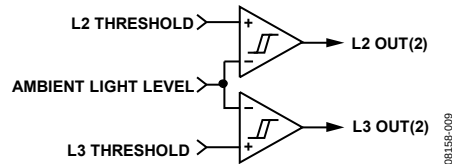
Figure 9. Light Sensing Comparators
