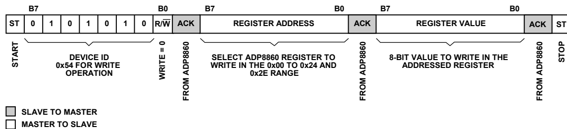
Figure 3. I 2 C Write Operation
