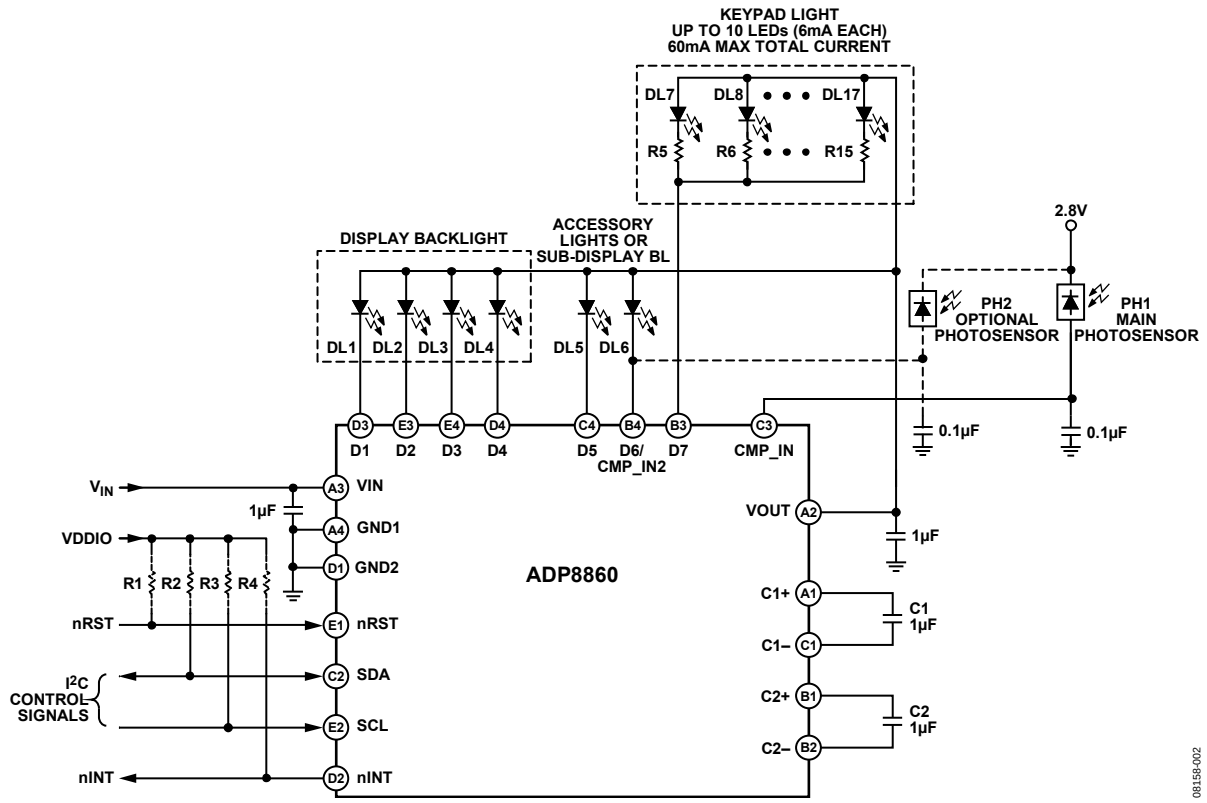
Figure 2. Schematic with Keypad Light Control
