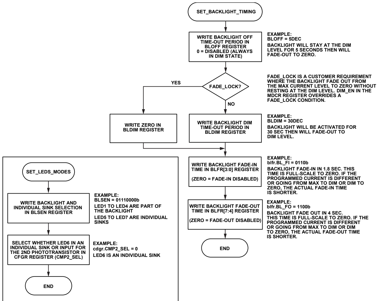
Figure 11. Set Backlight Timing Flowchart
