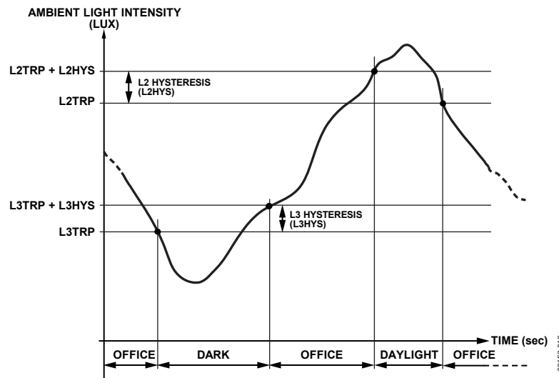
Figure 10. Comparator Thresholds
