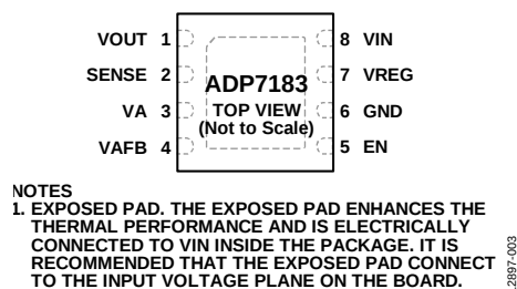
Figure 3. Pin Configuration
