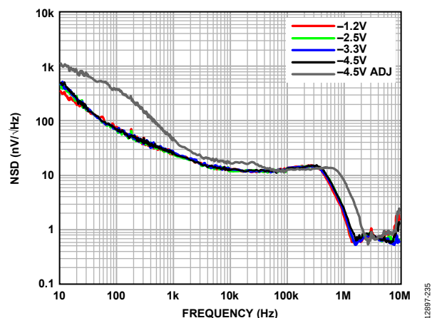
Figure 35. Noise Spectral Density (NSD) vs. Frequency at Various Output Voltages
