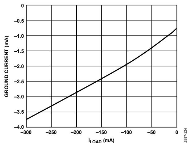
Figure 14. Ground Current vs. Load Current ( I_{LOAD} ), V_{OUT} = -2.5\text{ V}
