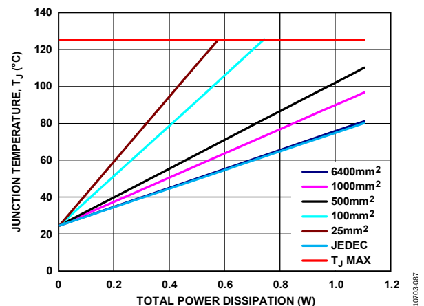
Figure 89. Junction Temperature vs. Total Power Dissipation for the 8-Lead LFCSP, T_A = 25^\circ\text{C}
