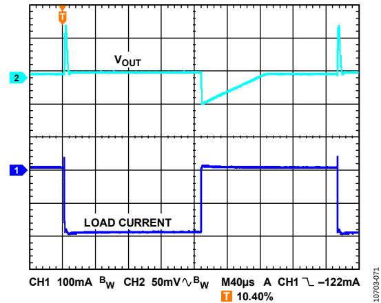
Figure 73. Load Transient Response, V_{OUT} = -1.22 V, I_{LOAD} = -1 mA to -200 mA, Load Step = 1 A/μs
