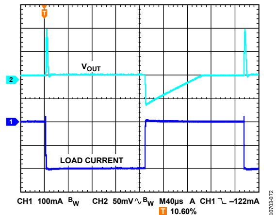
Figure 74. Load Transient Response, V_{OUT} = -3 V, I_{LOAD} = -1 mA to -200 mA, Load Step = 1 A/μs
