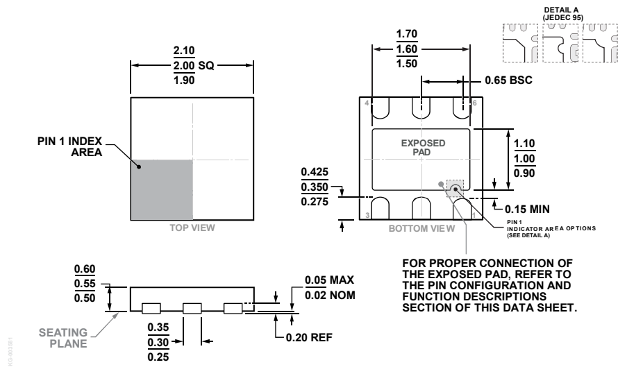
Figure 104. 6-Lead Lead Frame Chip Scale Package [LFCSP] 2.00 mm × 2.00 mm Body and 0.55 Package Height (CP-6-3)
