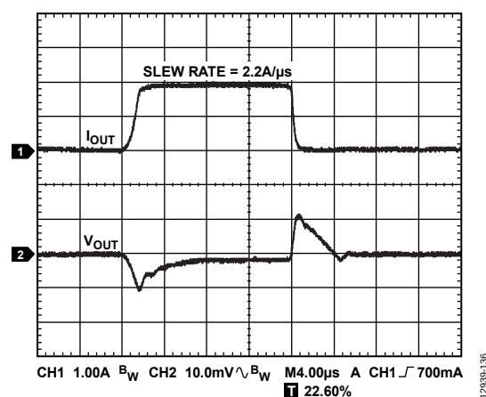
Figure 34. Load Transient Response, I_{LOAD} = 100\text{mA} to 2 A, V_{OUT} = 3.3\text{V} , V_{IN} = 4.0\text{V} , C_{OUT} = 22\mu\text{F} , Channel 1 = I_{OUT} , Channel 2 = V_{OUT}
