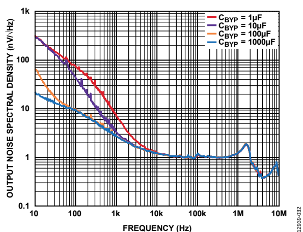
Figure 30. Output Noise Spectral Density vs. Frequency at Various Values of C_{BYP}
