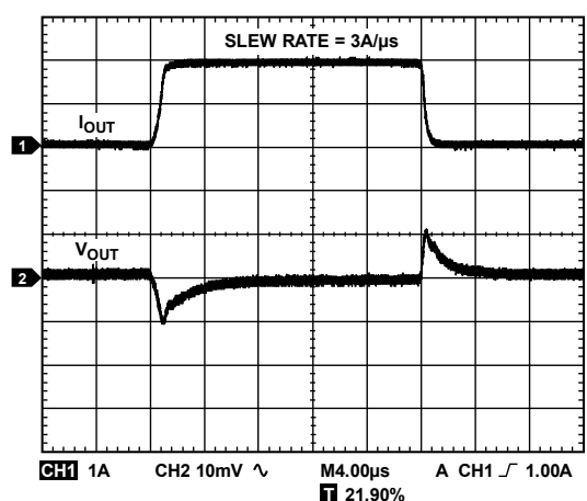
Figure 33. Load Transient Response, I_{LOAD} = 100\text{mA} to 2 A, V_{OUT} = 3.3\text{V} , V_{IN} = 4.0\text{V} , Channel 1 = I_{OUT} , Channel 2 = V_{OUT}
