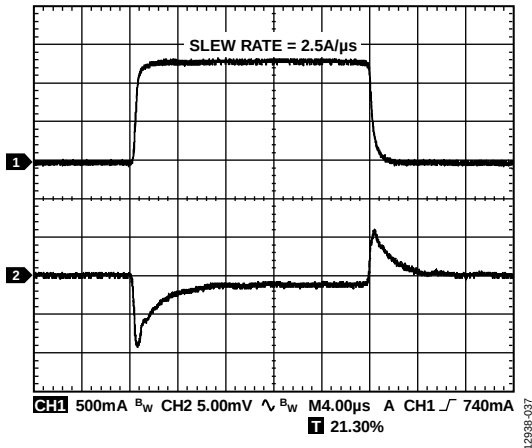
Figure 35. Load Transient Response, I_{LOAD} = 100\text{ mA} to 1.2\text{ A} , V_{OUT} = 1.8\text{ V} , V_{IN} = 2.5\text{ V} , Channel 1 = I_{OUT} , Channel 2 = V_{OUT}
