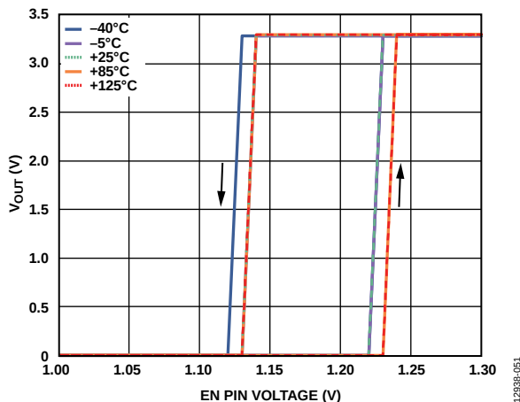
Figure 49. Typical VOUT Response to EN Pin Operation
