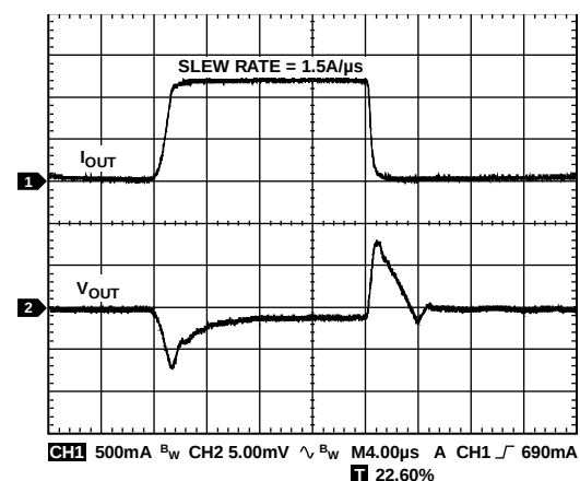
Figure 34. Load Transient Response, I_{LOAD} = 100 \text{ mA} to 1.2 \text{ A} , V_{OUT} = 3.3 \text{ V} , V_{IN} = 4.0 \text{ V} , C_{OUT} = 22 \mu\text{F} , Channel 1 = I_{OUT} , Channel 2 = V_{OUT}
