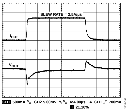
Figure 44. Output Transient Response, V_{OUT} = 3.3\text{ V} , C_{OUT} = 10\text{ }\mu\text{F} , Channel 1 = Load Current, Channel 2 = V_{OUT}
