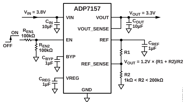
Figure 52. Typical EN Pin Voltage Divider
