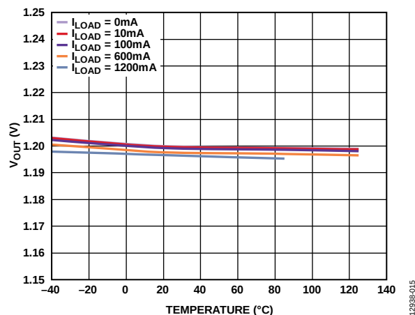
Figure 15. Output Voltage ( V_{OUT} ) vs. Temperature at Various Loads, V_{OUT} = 1.2\text{ V}
