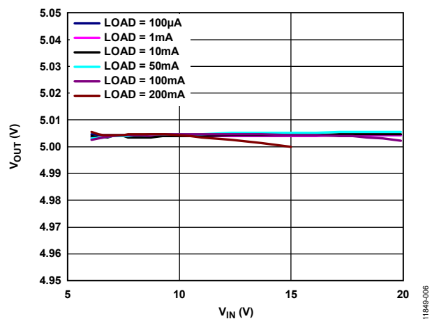
Figure 8. Output Voltage ( V_{OUT} ) vs. Input Voltage ( V_{IN} )
