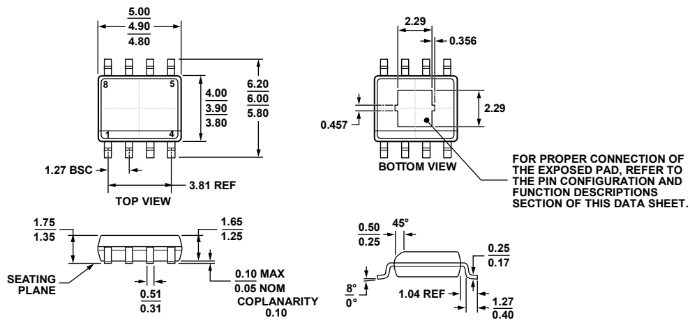
COMPLIANT TO JEDEC STANDARDS MS-012-AA Figure 68. 8-Lead Standard Small Outline Package, with Exposed Pad [SOIC_N_EP] Narrow Body (RD-8-1)
