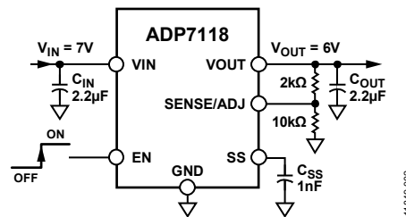
Figure 2. ADP7118 with 5 V Output Adjusted to 6 V
