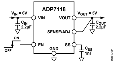
Figure 1. ADP7118 with Fixed Output Voltage, 5 V
