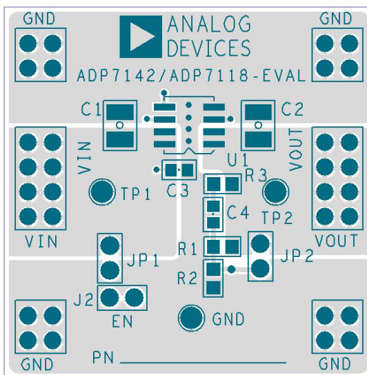
Figure 65. Example SOIC PCB Layout
