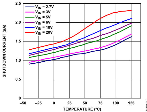
Figure 12. Shutdown Current vs. Temperature at Various Input Voltages
