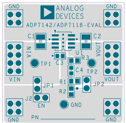
Figure 3. ADP7118/ADP7142 SOIC Evaluation Board
