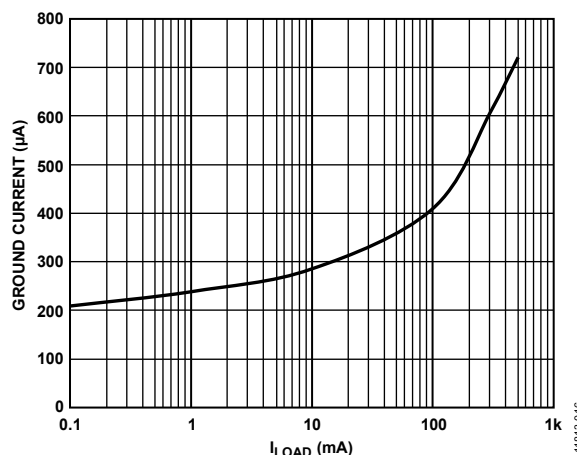
Figure 16. Ground Current vs. Load Current ( I_{LOAD} )
