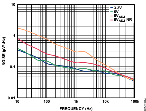
Figure 49. Output Noise Spectral Density, I_{LOAD} = 10\text{ mA} , C_{OUT} = 1\text{ }\mu\text{F}
