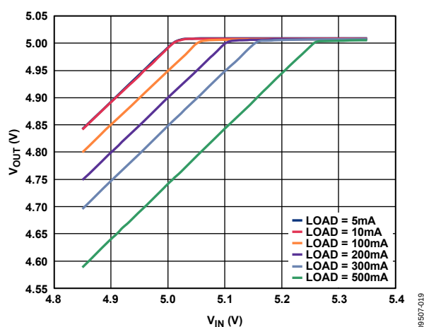
Figure 21. Output Voltage vs. Input Voltage (in Dropout)
