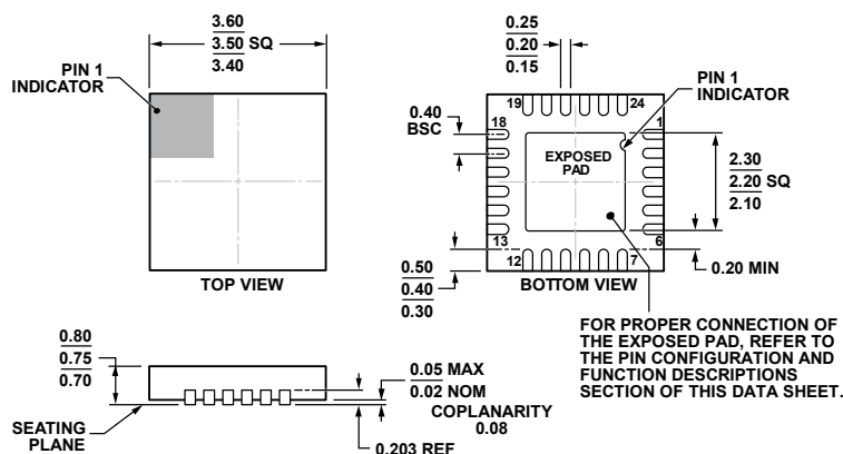
Figure 32. 24-Lead Lead Frame Chip Scale Package [LFCSP_WQ] 3.5 mm × 3.5 mm Body, Very Very Thin Quad (CP-24-11)
