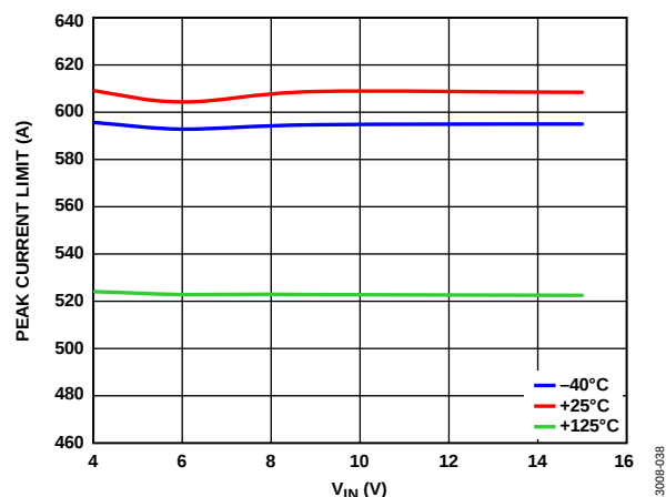
Figure 38. Channel 2 Peak Current Limit vs. V_{IN}
