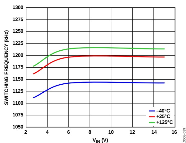
Figure 39. Switching Frequency vs. V_{IN}
