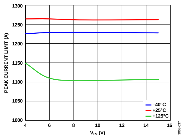
Figure 37. Channel 1 Peak Current Limit vs. V_{IN}
