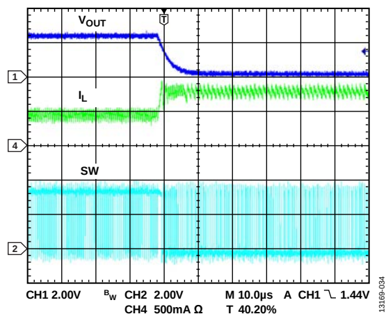
Figure 34. Output Short
