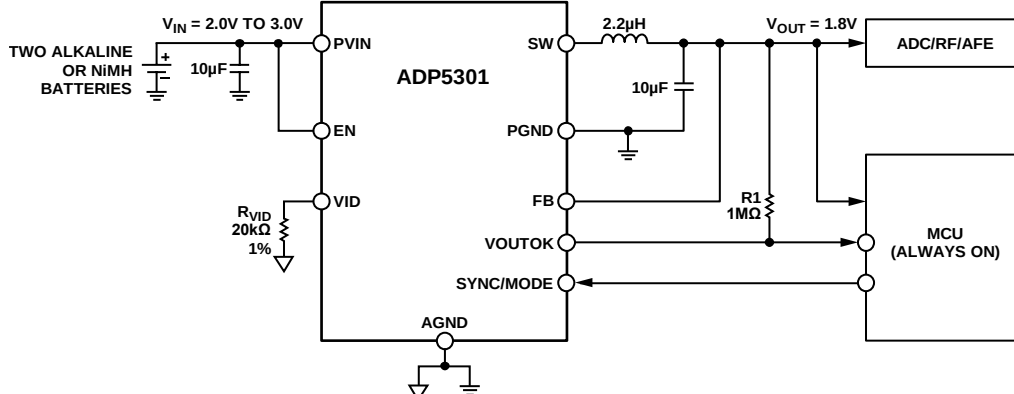
Figure 41. Typical ADP5301 Application with Two Alkaline/NiMH Batteries
