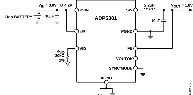
Figure 40. Typical ADP5301 Application with Li-Ion Battery
