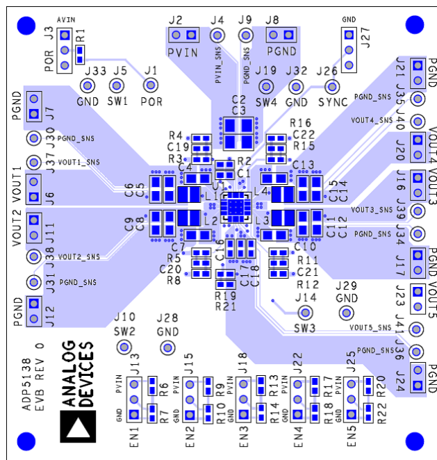
Figure 4. Layer 1, Component Side
