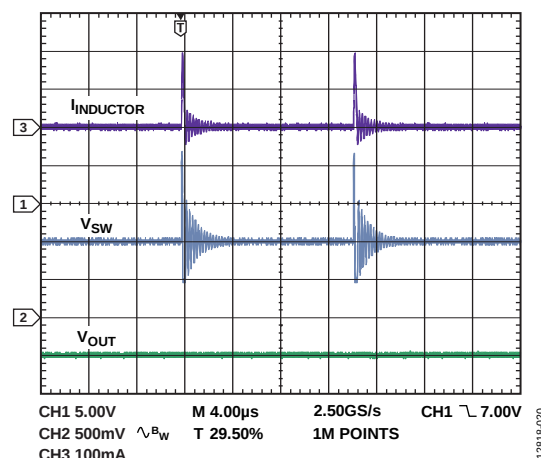
Figure 18. Skip Mode Operation Showing Inductor Current ( I_{INDUTOR} ), Switch Node Voltage ( V_{SW} ), and Output Ripple ( V_{OUT} ), V_{IN} = 12\text{ V} , V_{OUT} = -5\text{ V} , I_{LOAD} = 1\text{ mA} , f_{SW} = 1.2\text{ MHz} , T_A = 25^\circ\text{C}
