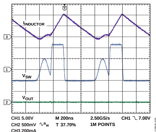
Figure 19. Discontinuous Conduction Mode Operation Showing Inductor Current ( I_{INDUTOR} ), Switch Node Voltage ( V_{SW} ), and Output Ripple ( V_{OUT} ), V_{IN} = 12\text{ V} , V_{OUT} = -5\text{ V} , I_{LOAD} = 100\text{ mA} , f_{SW} = 1.2\text{ MHz} , T_A = 25^\circ\text{C}
