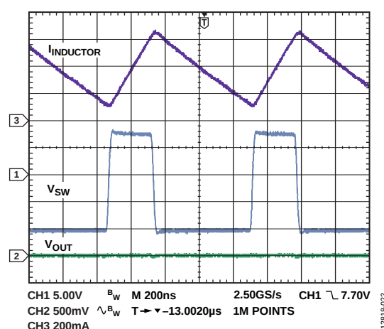
Figure 20. Continuous Conduction Mode Operation Showing Inductor Current ( I_{INDUTOR} ), Switch Node Voltage ( V_{SW} ), and Output Ripple ( V_{OUT} ), V_{IN} = 12\text{ V} , V_{OUT} = -5\text{ V} , I_{LOAD} = 250\text{ mA} , f_{SW} = 1.2\text{ MHz} , T_A = 25^\circ\text{C}
