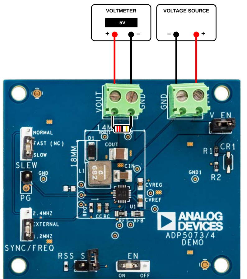
Figure 3. Output Voltage Measurement
