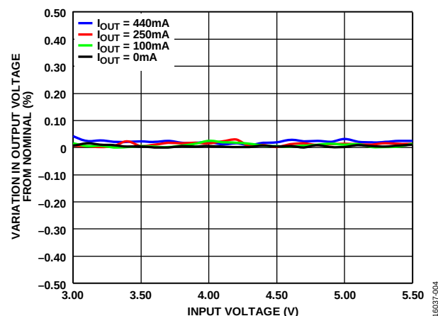
Figure 5. ADP5073 Line Regulation, V_{NEG} = -5\text{V} , f_{SW} = 2.4\text{MHz} , T_A = 25^\circ\text{C}
