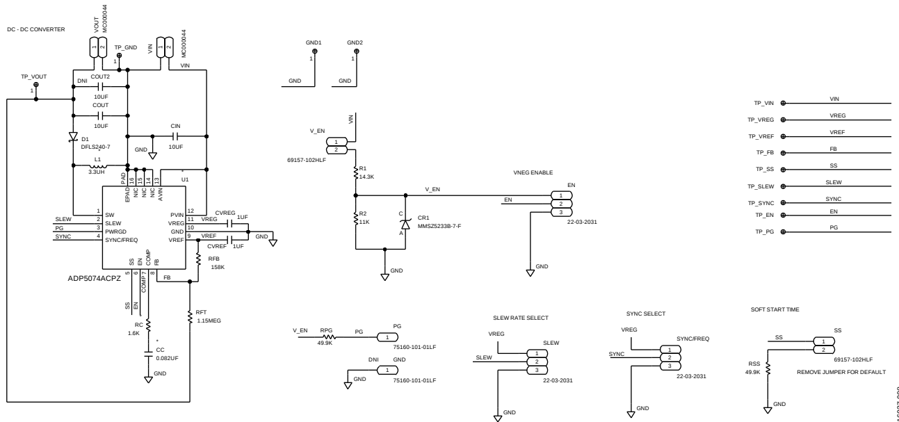
Figure 9. Evaluation Board Schematic for the ADP5074
