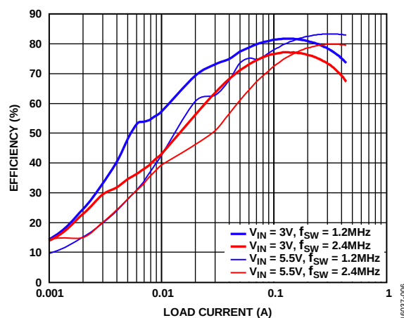
Figure 7. ADP5073 Efficiency vs. Load Current, V_{NEG} = -5\text{V} , T_A = 25^\circ\text{C}
