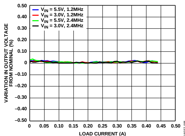
Figure 6. ADP5073 Load Regulation, V_{NEG} = -5\text{V} , T_A = 25^\circ\text{C}
