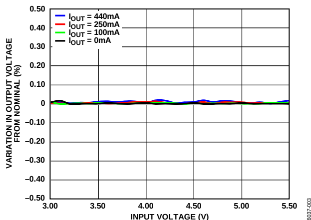
Figure 4. ADP5073 Line Regulation, V_{NEG} = -5\text{V} , f_{SW} = 1.2\text{MHz} , T_A = 25^\circ\text{C}
