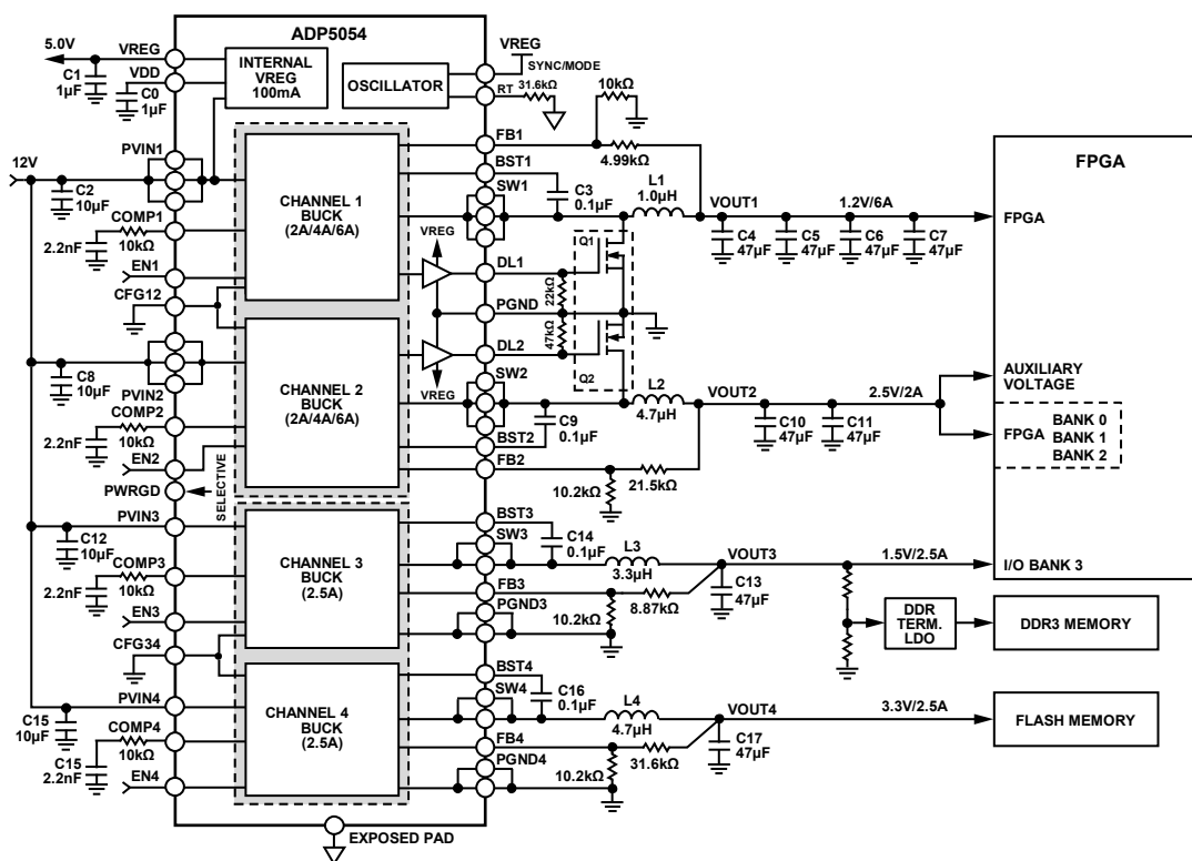
Figure 44. Typical Field Programmable Gate Array (FPGA) Application, 600 kHz Switching Frequency, Adjustable Output Model
