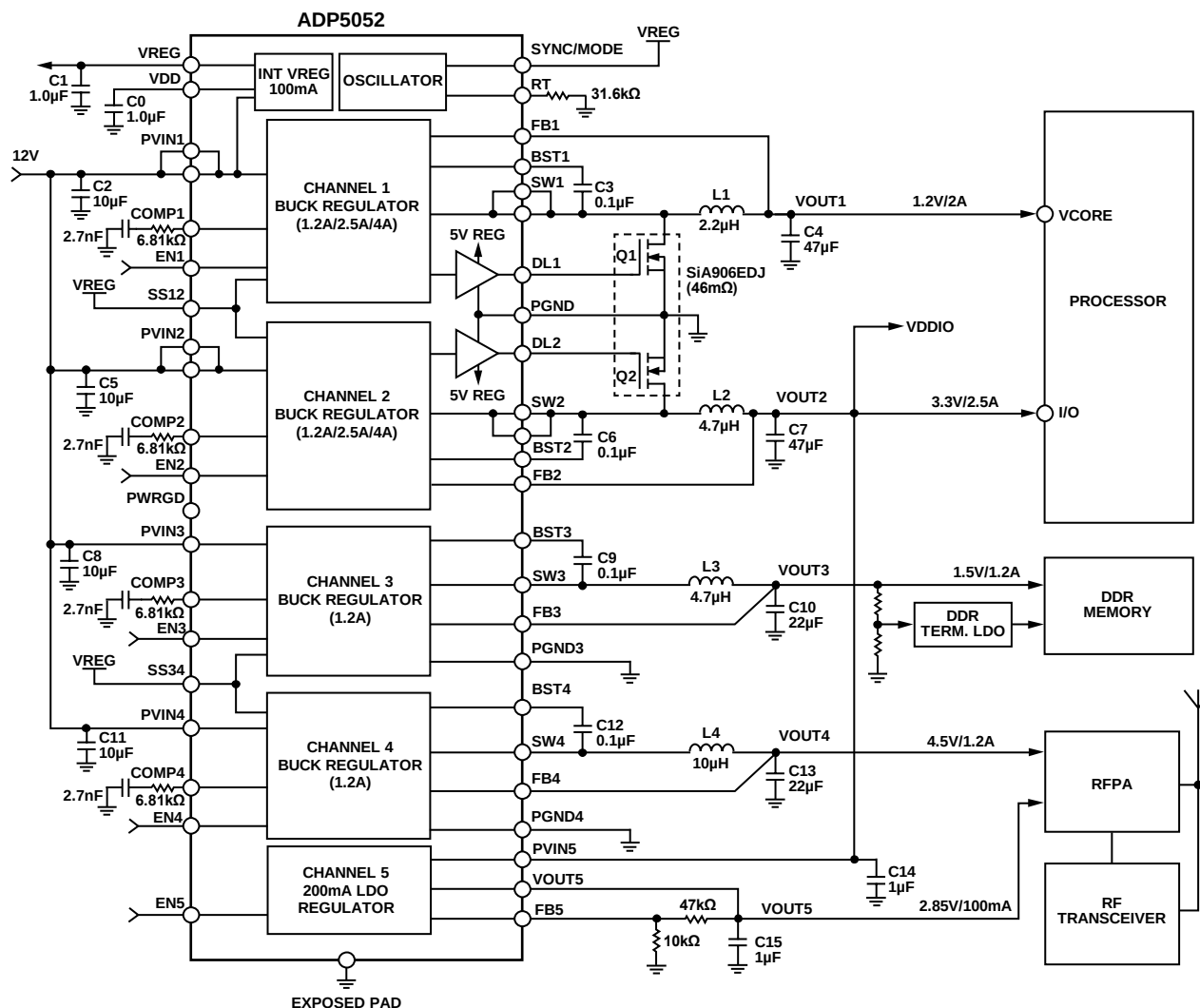
Figure 54. Typical Femtocell Application, 600 kHz Switching Frequency, Fixed Output Model
