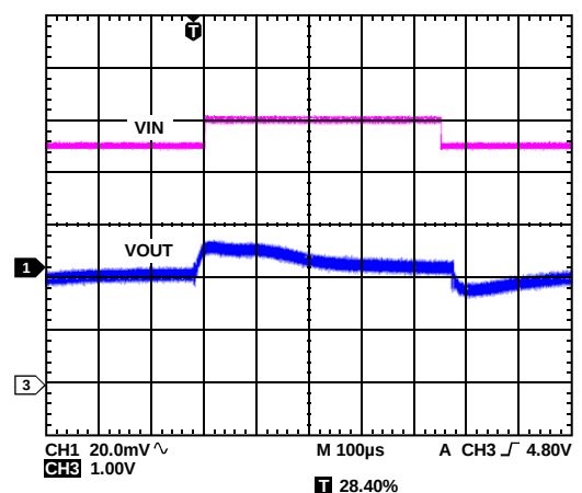
Figure 38. LDO Response to Line Transient, Input Voltage from 4.5 V to 5 V, V_{OUT3} = 2.8\text{ V}
