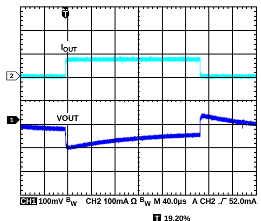
Figure 37. LDO Response to Load Transient, I_{OUT3} from 1 mA to 80 mA, V_{OUT3} = 2.8\text{ V}
