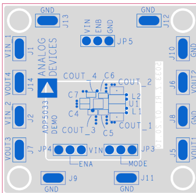
Figure 12. Bottom Layer, Recommended Layout
