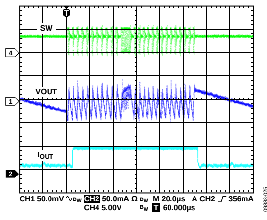
Figure 25. BUCK1 Response to Load Transient, I_{OUT1} from 1\text{ mA} to 50\text{ mA} , V_{OUT1} = 3.3\text{ V} , Automatic Mode
