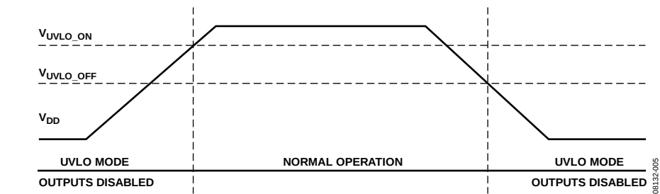
Figure 5. UVLO Function
