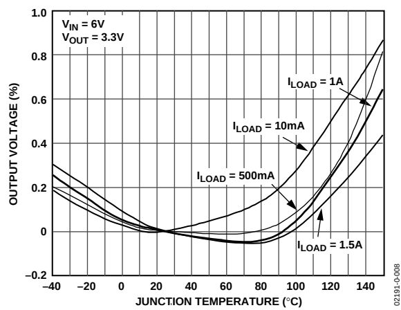
Figure 8. Output Voltage Variation Percentage vs. Junction Temperature
