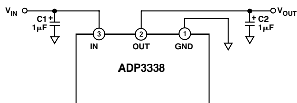
Figure 3. Typical Application Circuit
