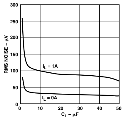
TPC 15. RMS Noise vs. C_L (10 Hz–100 kHz)
