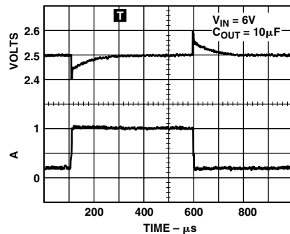
TPC 12. Load Transient Response
