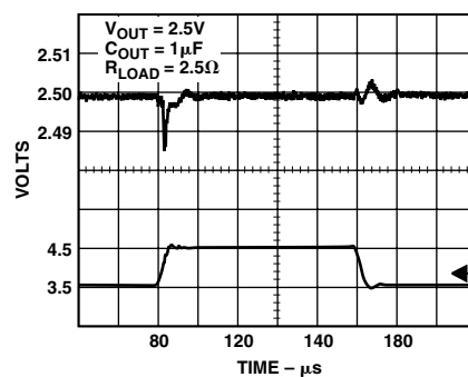
TPC 9. Line Transient Response
