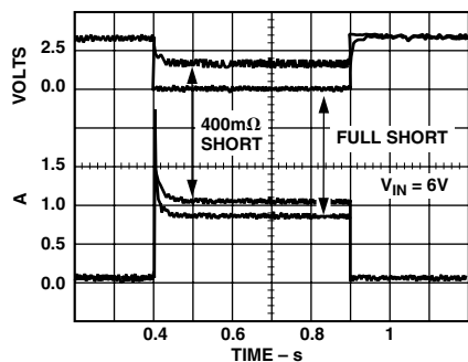
TPC 13. Short-Circuit Current
