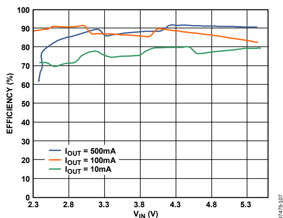
Figure 11. Efficiency vs. Input Voltage ( V_{OUT} = 3.3\text{ V} )
