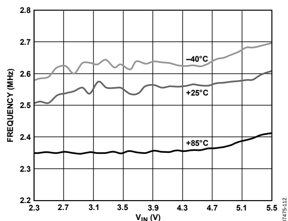
Figure 13. Frequency vs. Input Voltage Over Temperature ( V_{OUT} = 3.3\text{ V} )
