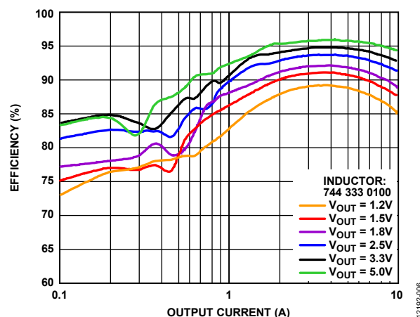
Figure 6. ADP2390 Efficiency at V_{PVIN} = 12\text{ V} , f_{SW} = 600\text{ kHz}
