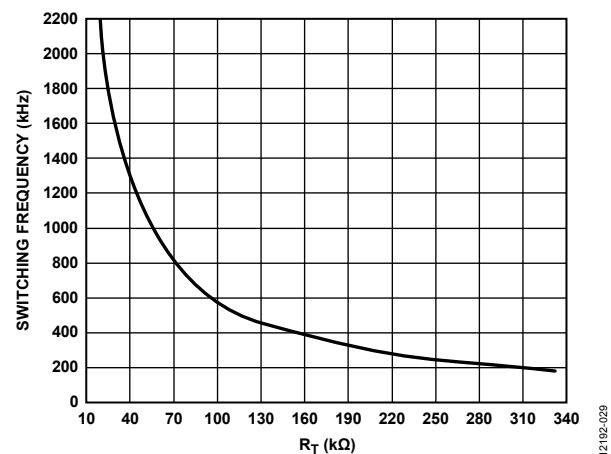
Figure 29. Switching Frequency ( f_{sw} ) vs. R_T
