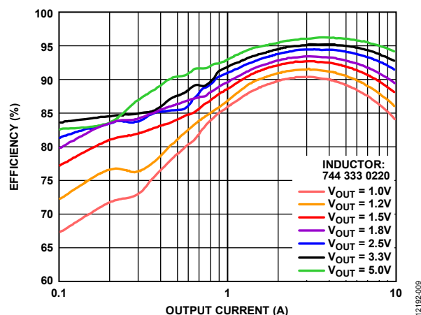
Figure 9. ADP2390 Efficiency at V_{PVIN} = 12\text{ V} , f_{SW} = 300\text{ kHz}
