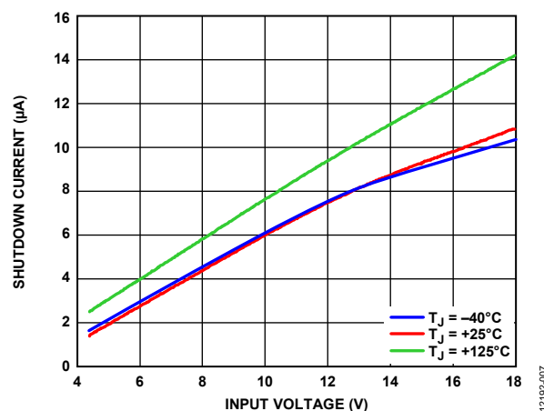
Figure 7. Shutdown Current ( I_{SHDN} ) vs. Input Voltage
