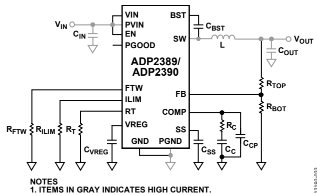
Figure 33. High Current Path in the PCB Circuit
