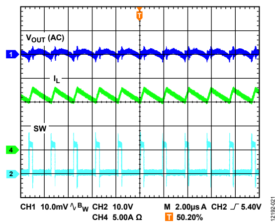
Figure 21. Continuous Conduction Mode (CCM) Waveform
