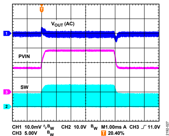
Figure 27. Line Transient Response, V_{VIN} from 8\text{ V} to 14\text{ V} , I_{OUT} = 12\text{ A}
