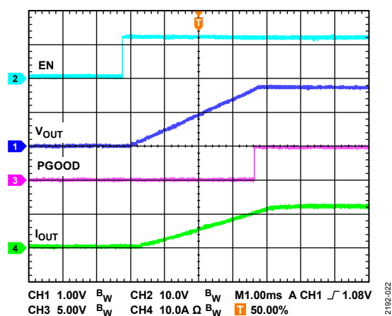
Figure 22. Soft Start with Full Load
