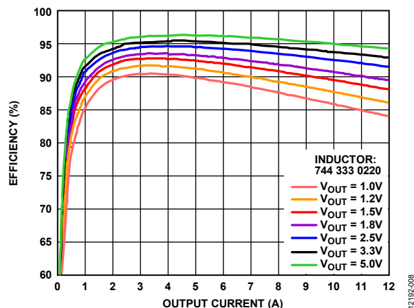
Figure 8. ADP2389 Efficiency at V_{PVIN} = 12\text{ V} , f_{SW} = 300\text{ kHz}
