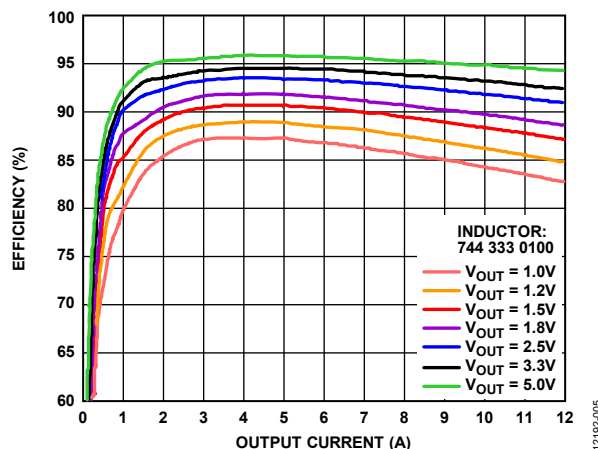
Figure 5. ADP2389 Efficiency at V_{PVIN} = 12\text{ V} , f_{SW} = 600\text{ kHz}
