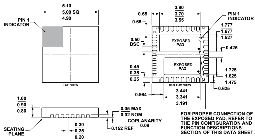
Figure 38. 32-Lead Lead Frame Chip Scale Package [LFCSP_VQ] 5 mm x 5 mm Body, Very Thin Quad (CP-32-19) Dimensions shown in millimeters
