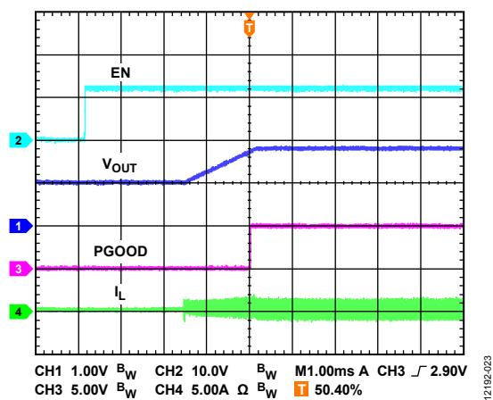
Figure 23. Precharged Output
