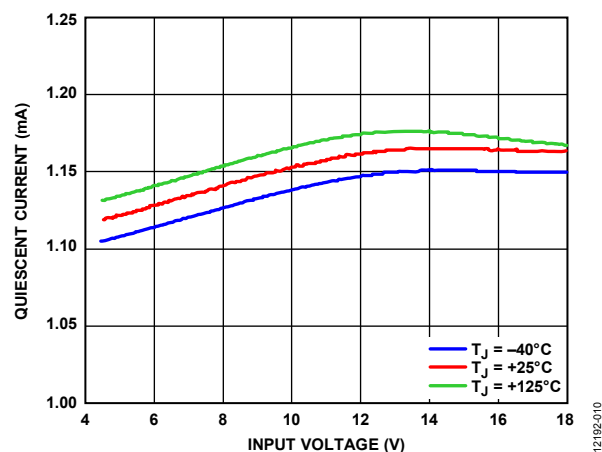
Figure 10. Quiescent Current ( I_Q ) vs. Input Voltage
