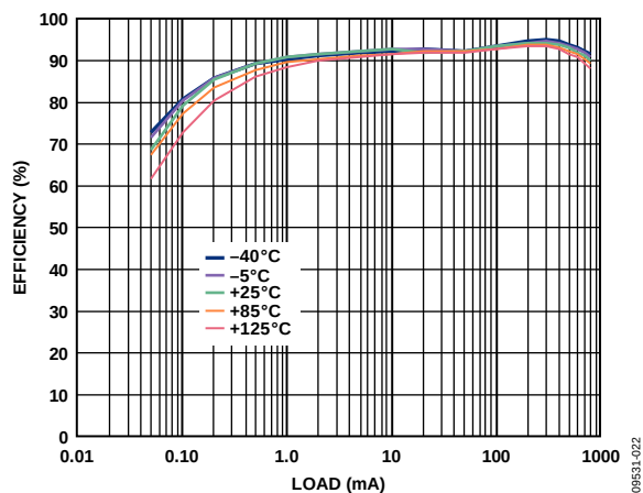
Figure 22. Efficiency vs. Load Current, V_{OUT} = 5.0 V, Different Temperatures
