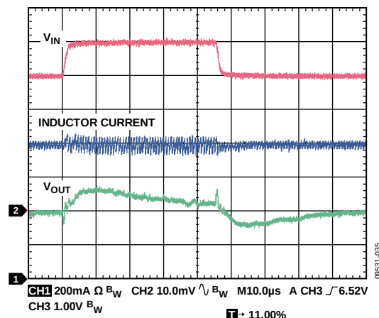
Figure 35. Line Transient, V_{OUT} = 5V , PWM Mode, 800 mA, V_{IN1} = 6V to 7V , 2\mu s Rise Time, C_{IN} = 3.3\mu F
