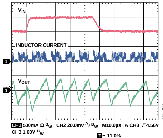
Figure 30. Line Transient, V_{OUT} = 1.2\text{ V} , PSM Mode, 100 mA, V_{IN1} = 4\text{ V} to 5\text{ V} , 2\text{ }\mu\text{s} Rise Time, C_{IN} = 3.3\text{ }\mu\text{F}
