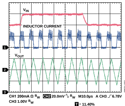
Figure 32. Line Transient, V_{OUT} = 3.3\text{ V} , PSM Mode, 100 mA, V_{IN1} = 6\text{ V} to 7\text{ V} , 2\text{ }\mu\text{s} Rise Time, C_{IN} = 3.3\text{ }\mu\text{F}
