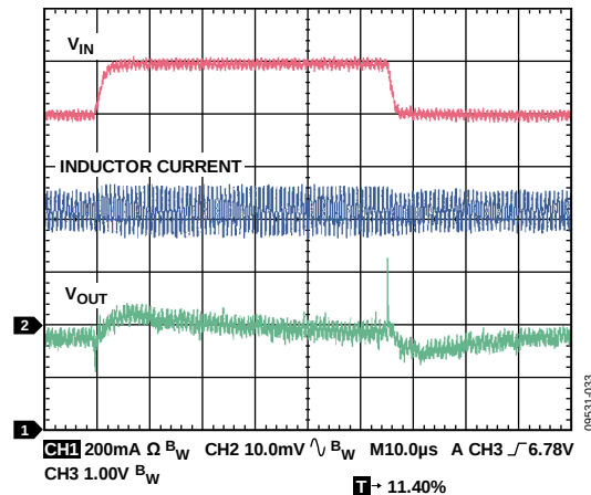
Figure 33. Line Transient, V_{OUT} = 3.3V , PWM Mode, 800 mA, V_{IN1} = 6V to 7V , 2\mu s Rise Time, C_{IN} = 3.3\mu F
