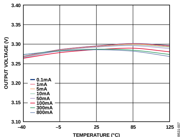
Figure 7. Output Voltage vs. Temperature, V_{OUT} = 3.3\text{ V} , V_{IN} = 7.3\text{ V} , Different Loads
