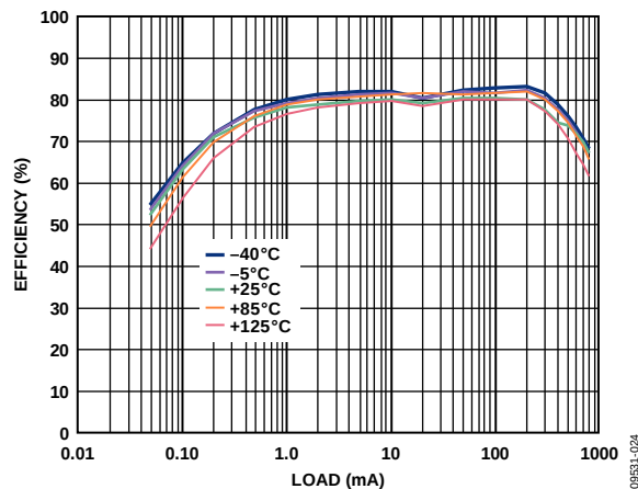
Figure 24. Efficiency vs. Load Current, V_{OUT} = 1.2 V, Different Temperatures, V_{IN} = 4 V
