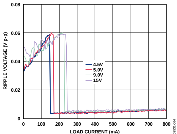
Figure 64. Output Ripple vs. Load Current, V_{OUT} = 3.3\text{ V} , Different Input Voltages, Automatic Mode
