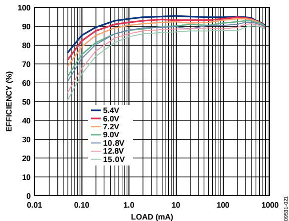
Figure 21. Efficiency vs. Load Current, V_{OUT} = 5.0 V, Different Input Voltages
