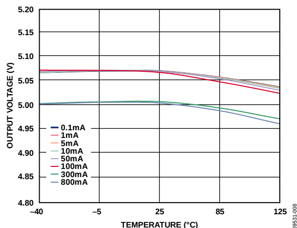
Figure 8. Output Voltage vs. Temperature, V_{OUT} = 5\text{ V} , V_{IN} = 7.2\text{ V} , Different Loads
