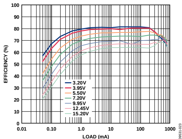
Figure 23. Efficiency vs. Load Current, V_{OUT} = 1.2 V, Different Input Voltages
