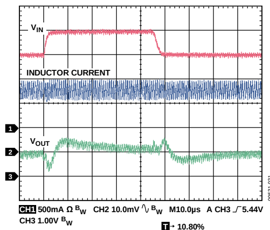
Figure 31. Line Transient, V_{OUT} = 1.2\text{ V} , PWM Mode, 800 mA, V_{IN1} = 4\text{ V} to 5\text{ V} , 2\text{ }\mu\text{s} Rise Time, C_{IN} = 3.3\text{ }\mu\text{F}
