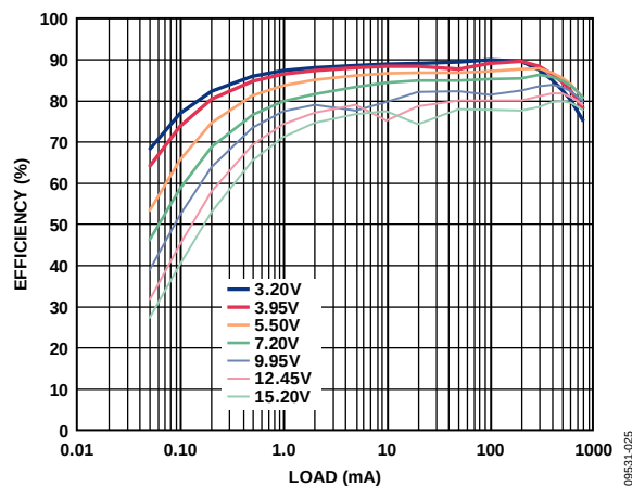
Figure 25. Efficiency vs. Load Current, V_{OUT} = 1.8 V, Different Input Voltages
