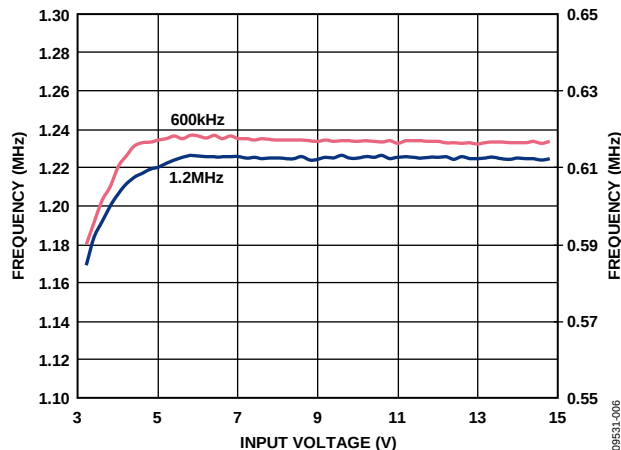
Figure 6. Switching Frequency vs. Input Voltage, FPWM Mode
