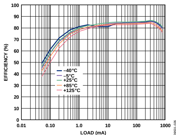
Figure 26. Efficiency vs. Load Current, V_{OUT} = 1.8 V, Different Temperatures, V_{IN} = 4 V
