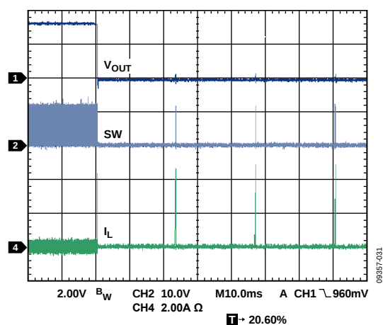
Figure 31. Output Short
