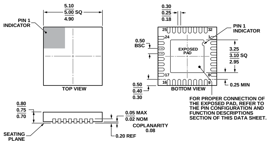
Figure 58. 32-Lead Lead Frame Chip Scale Package [LFCSP_WQ] 5 mm × 5 mm Body, Very Very Thin Quad (CP-32-7) Dimensions shown in millimeters
