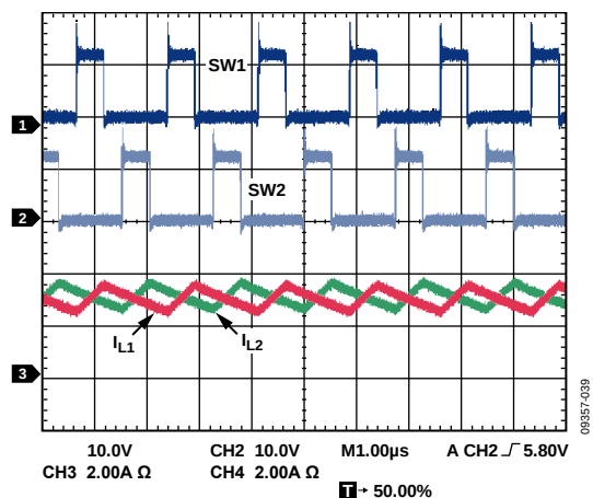
Figure 39. Dual Phase, Single Output, V_{OUT} = 3.3\text{ V} , I_{OUT} = 6\text{ A}
