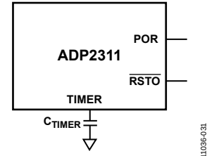
Figure 31. Capacitor Connected Between TIMER and GND
