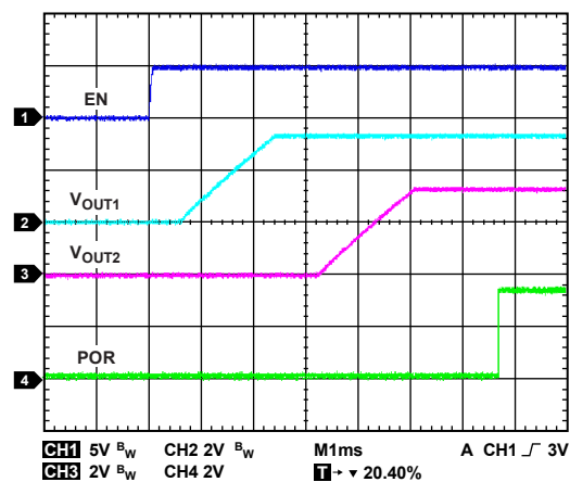
Figure 27. Soft Start with Full Load
