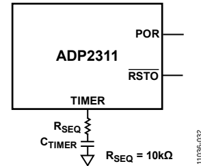
Figure 32. Resistor and Capacitor Connected Between TIMER and GND
